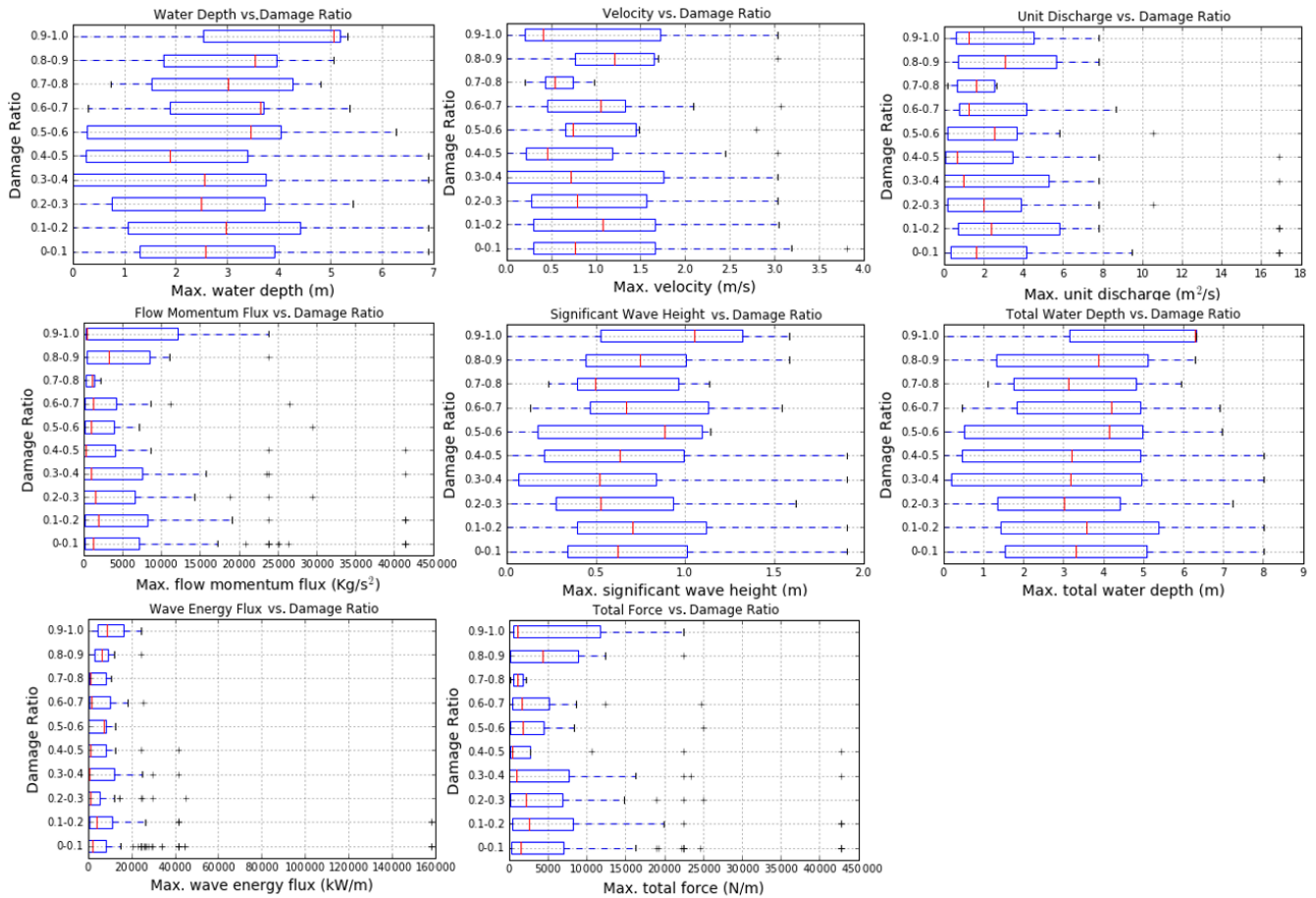
Figure A1. Box-whisker plots for the variables ( h , v , hv , \rho hv^2 , H_{\text{sig}} , h + H_{\text{sig}} , E_f , \frac{E_f}{C_g} + \rho hv^2 ) with the GEBCO DEM.
