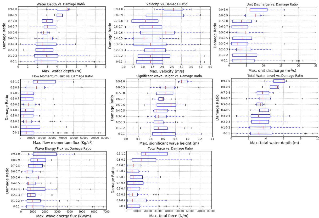
Figure A3. Box-whisker plots for the variables ( h , v , hv , \rho hv^2 , H_{\text{sig}} , h + H_{\text{sig}} , E_f , \frac{E_f}{C_g} + \rho hv^2 ) with the IGN + structures DEM.
