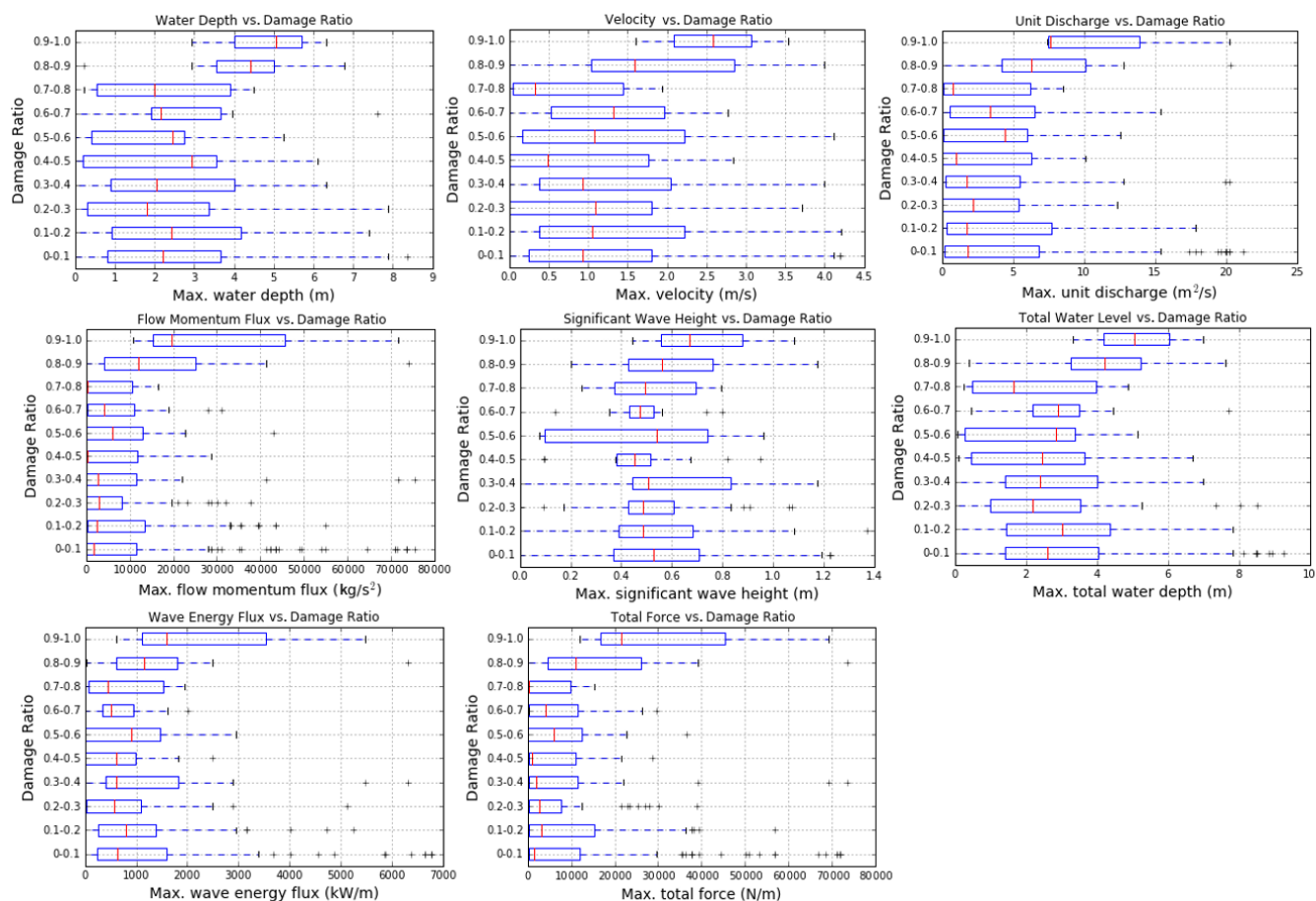
Figure A2. Box-whisker plots for the variables ( h , v , hv , \rho hv^2 , H_{\text{sig}} , h + H_{\text{sig}} , E_f , \frac{E_f}{C_g} + \rho hv^2 ) with the IGN DEM.
