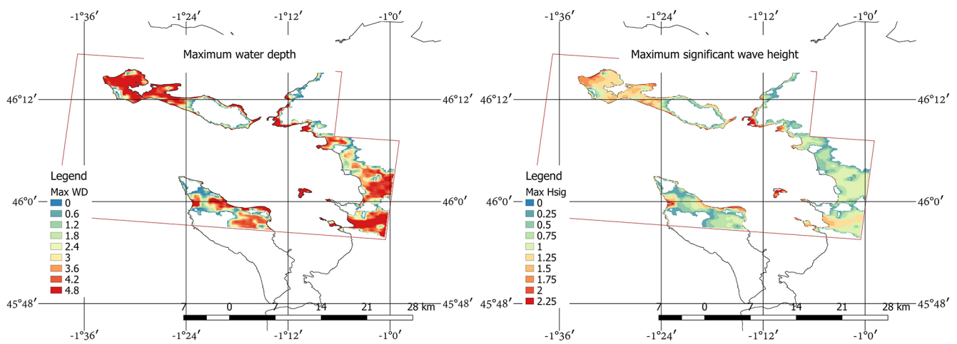
Figure 6. Maximum water level and maximum significant wave height ( H_{sig} ) footprints for the small model domain (case study area). Water depth and wave height are in units of metres. The purple rectangle indicates the limits of the small domain, outside of which data are not shown.
