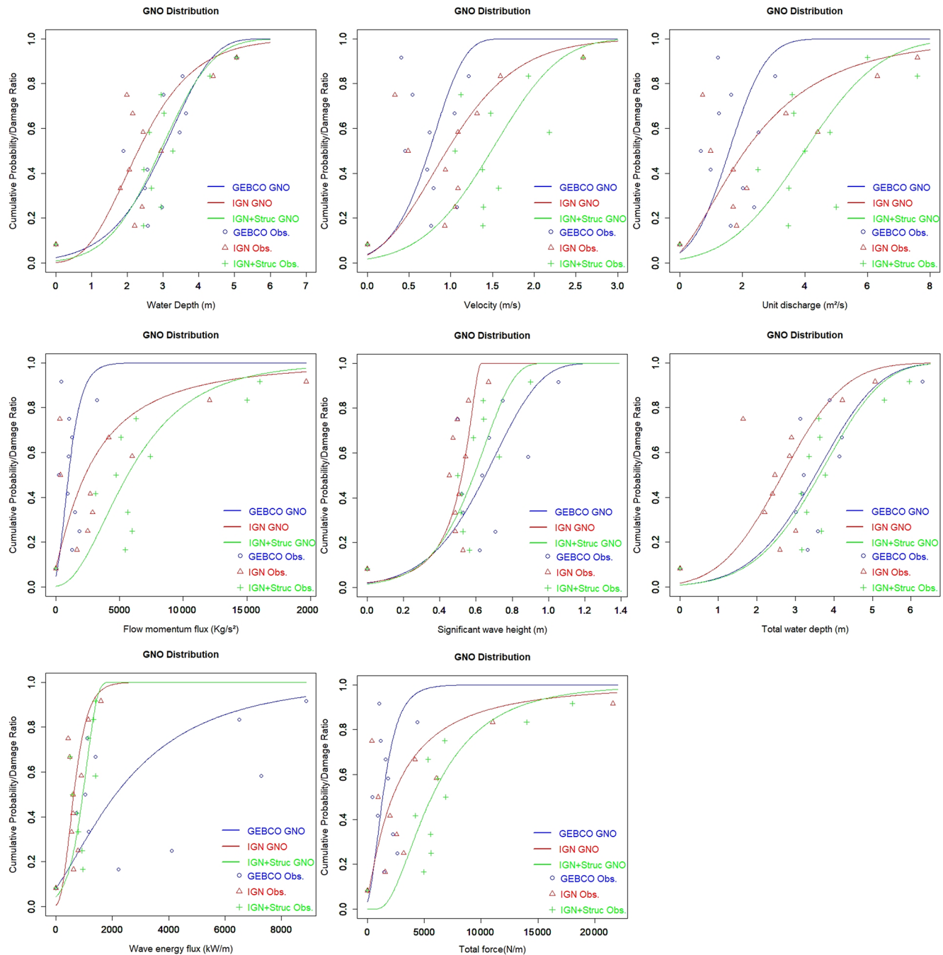
Figure 7. Damage curves for the surge and wave variables ( h, v, hv, \rho hv^2, H_{\text{sig}}, h + H_{\text{sig}}, E_f, \frac{E_f}{C_g} + \rho hv^2 ) and different bathymetry/topography conditions (Table 1). Markers indicate the observed data and lines the fitted statistical distributions.
