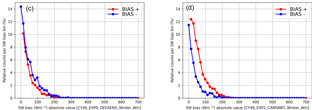
Figure 8. SW radiation bias ( \text{Wm}^{-2} ) for summer and winter 2-week periods for experiments with HARMONIE-AROME Cycle 46 over Ireland without NRT aerosols (Tegen) (a,c) and using the NRT aerosols (b,d).
