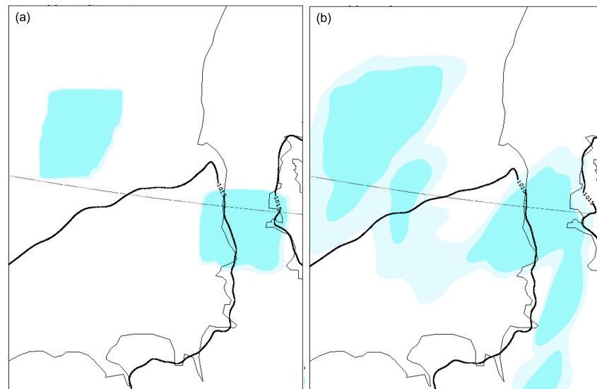
Figure 9. Example of spurious cirrus clouds. (a) original OCND2. (b) OCND2 with technical corrections. Clouds are shown as cyan shading. The figures are from a 13 h forecast starting from 00 Z on 16 April 2018.
