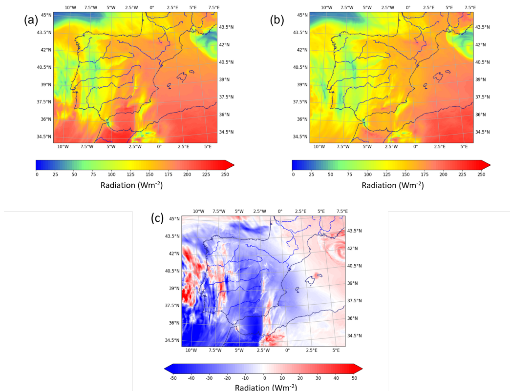
Figure 2. Dust case on the 20 of February 2023. Daily mean global SW radiation from HARMONIE-AROME Cycle 46 experiments. (a) using the default Tegen aerosol climatology, (b) using NRT CAMS aerosols, (c) difference between these.
