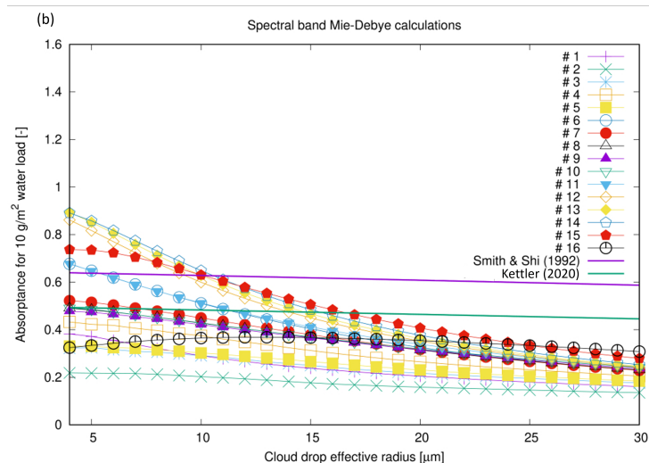
Figure 5. Spectral absorptance for a LWP of (a) 1 \text{ gm}^{-2} (b) and 10 \text{ gm}^{-2} for the 16 LW bands of the Nielsen scheme. Corresponding values calculated from the emissivity by the Smith and Shi [27] parametrization (purple continuous line) and the Kettler scheme (green continuous line [26]) are shown.
