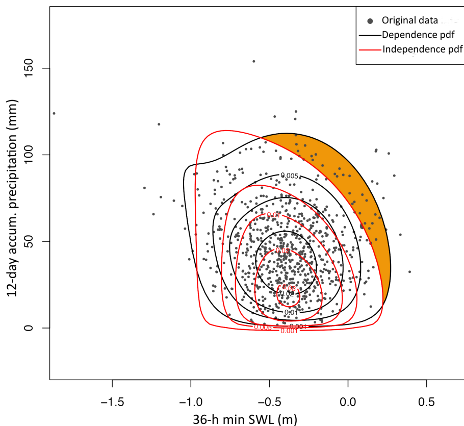
Figure 5. Scatter plot of S_{36\text{h,min}}^T and P_{12\text{d,acum}} and its joint PDF corresponding to original data (black) and shuffled data (red). Shaded orange area highlights the increased probability of extreme S_{36\text{h,min}}^T and P_{12\text{d,acum}} for the original data.
