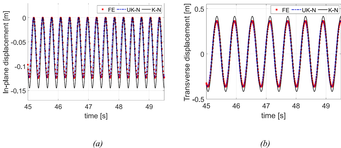
Fig. 3. Comparison of time domain response of a steel cantilever beam l = 0.6931 m, b = 0.0254 m, d = 0.99 mm obtained using full FEM, K-N and UK-N reduction – (a) in-plane tip displacement, (b) transverse tip displacement.
