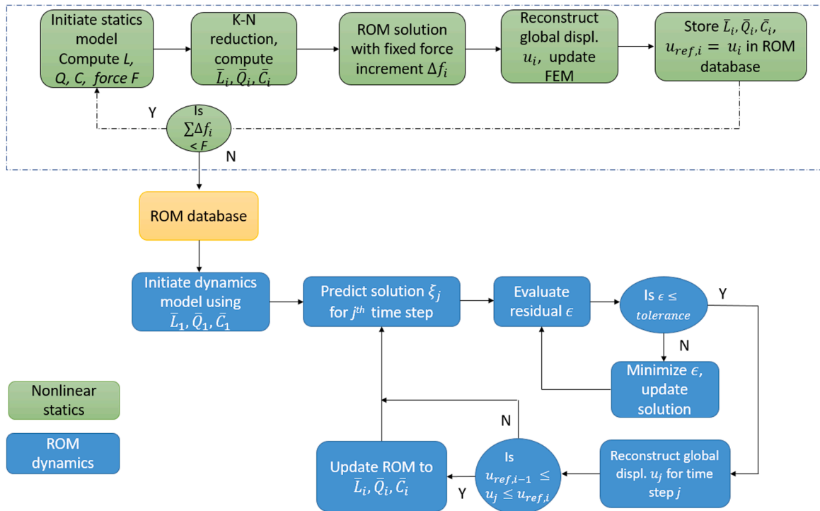
Fig. 2. Algorithm for the K-N reduction and updating procedure.
