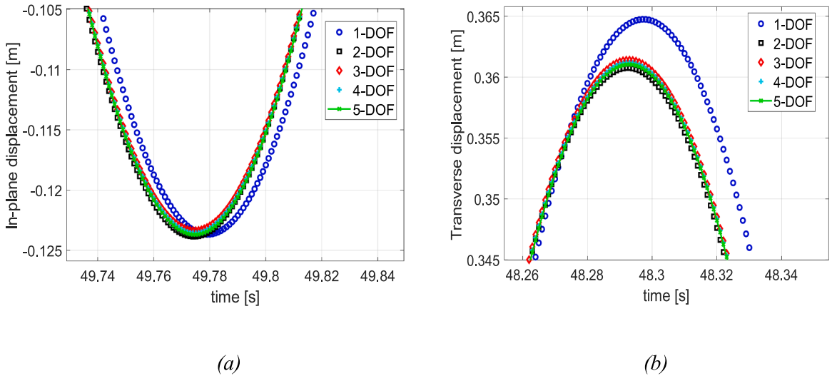
Fig 4. Magnified view of the time domain response of the steel cantilever beam l = 0.6931 m, b = 0.0254 m, d = 0.99 mm, obtained using various DOFs in the ROM for convergence analysis – (a) in-plane displacement, (b) transverse displacement.
