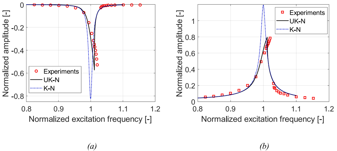
Fig 5. Comparison of K-N and UK-N based responses to experimental frequency response curves [10] of thin metal sheet l = 81.5 mm, b = 9 mm, d = 0.0762 mm – (a) in-plane displacement, (b) transverse displacement.
