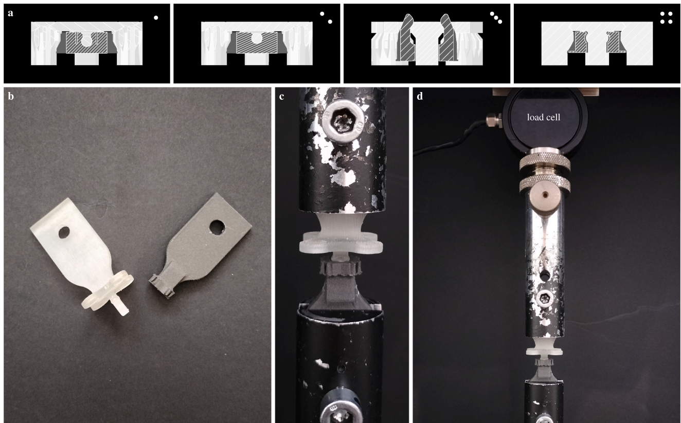
Fig. 3. The evaluation of the snapping mechanisms using a mechanical test setup to determine the required forces of the mechanism. a) Four examples, 1 to 4, of the different designs of the snapping mechanism to secure the lock in the locked position, after being pulled by a magnetic field. b) One of the four designs (specimen “4”) with the notch on the transparent part and the locking ring on the grey part. c) The specimen was initialized for the test with either part placed in one of the mounts. The locking ring was placed in the immobile lower mount, while the transparent part was placed in the moving upper mount. d) The upper part moved down for locking and up for release, as the load cell measured the applied force. The load cell was connected to the upper mount and provided quantifiable data regarding the performance of the design by measuring the force required to lock the mechanism.
