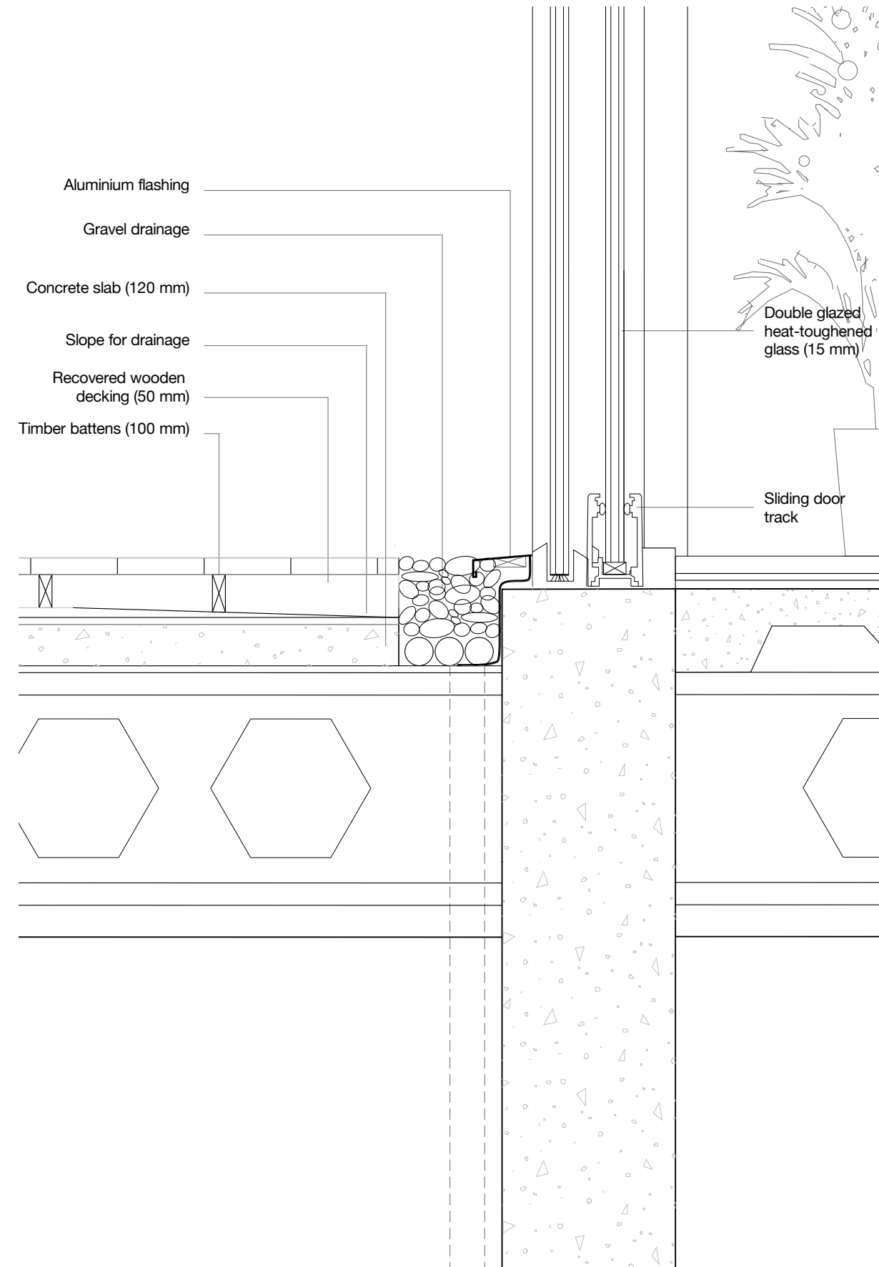
Detail B
