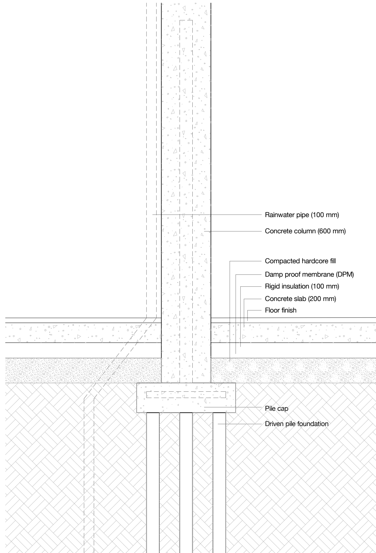
Detail A
