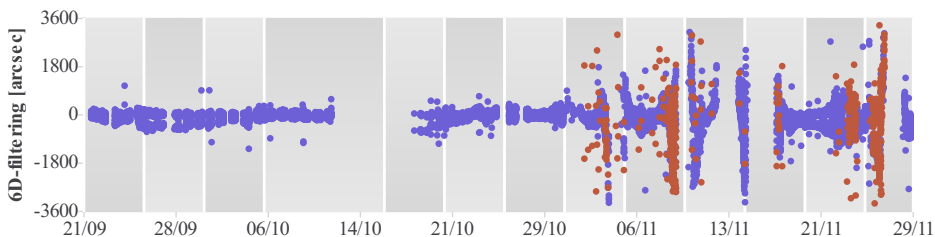
(c) Residuals of the 6D linear filtering over different data arcs represented by gray areas. Unprecise measurements due to coarse knowledge of the camera orientation are depicted in red.
