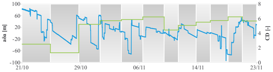
(a) Estimated relative semi-major axis (in blue) and chaser drag coefficient (in green).
