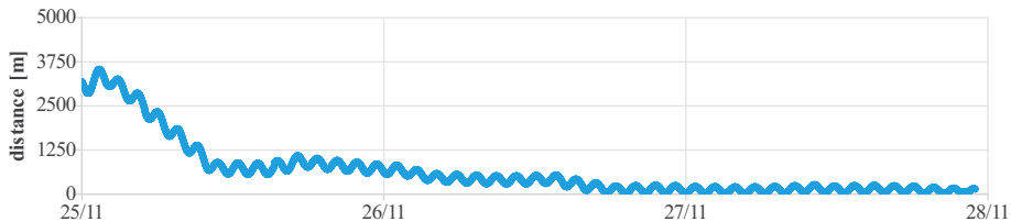
(a) Instantaneous intersatellite separation.
