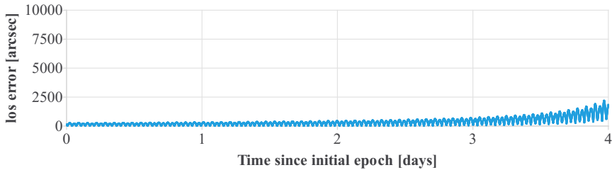
Figure 7.4: Measurement residuals obtained using the linear solution corrected for curved orbital path.
