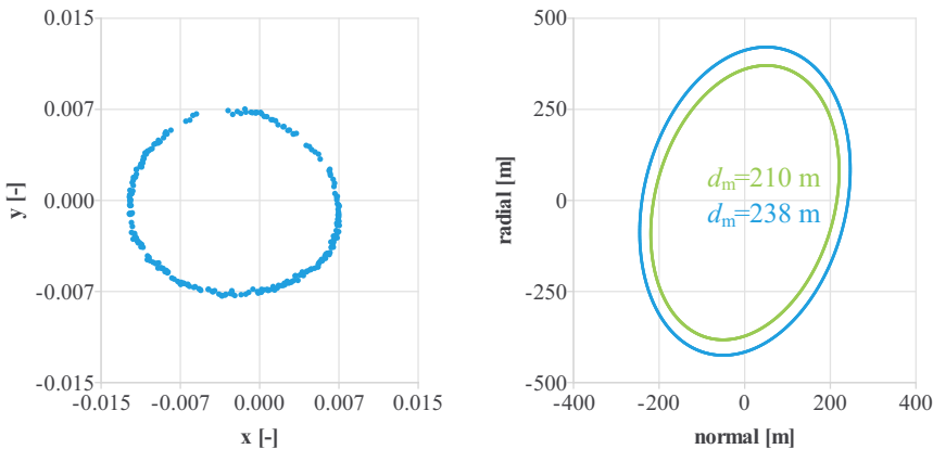
Figure 4.12: Relative orbit determination with a priori covariance at far-range (ARGON).
