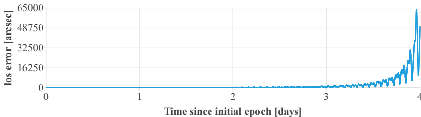
Figure 7.2: Measurement residuals obtained using the a priori solution x_0^{\text{apr}} .
