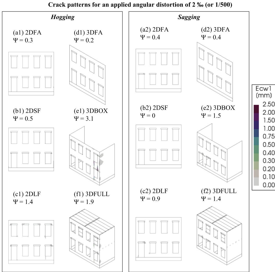
Figure 7. Resulting crack patterns for all the FE models at an applied angular distortion of 2 ‰ (or 1/500). The principal crack width ( E_{cw1} ) is shown. The damage parameter \Psi is reported for every model. (e1), (f1), (e2) and (f2) depict half the model.
