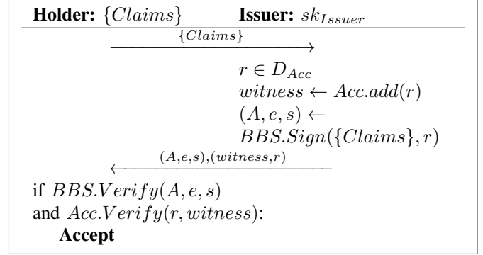
Protocol 1. Protocol of credential issuance.
