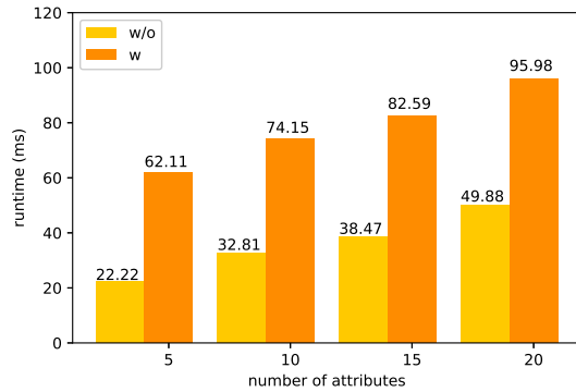
Fig. 4. Runtime measurements of verifiable credential presentation
