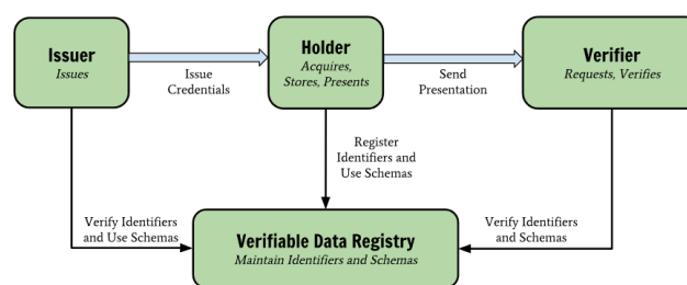
Fig. 1. Ecosystem of verifiable credentials.
