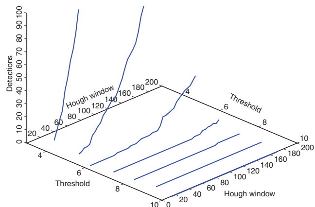
Figure 5. False-alarm rate as a function of HW and threshold. The HT detector is applied to the Fisher results of the synthetic noise. The false-alarm rate is higher if the threshold is lower and the HW is larger.
