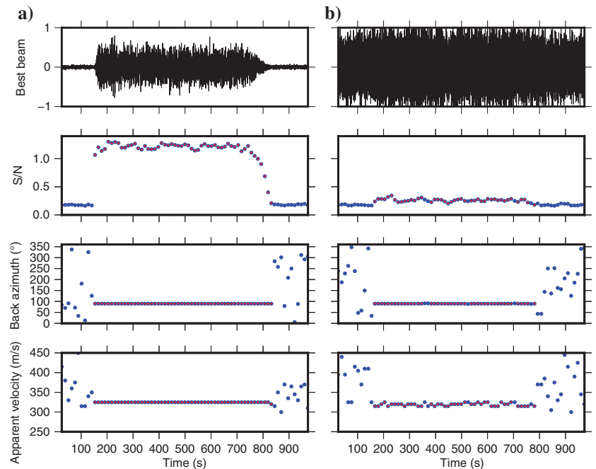
Figure 7. A synthetic long-duration signal with different S/N values. Columns A and B show a high- and a low-S/N signal, respectively. The frames from top to bottom show S/N, BA, and AV as a function of time. The blue and red dots are the Fisher and HT detector results, respectively. For the high-S/N signal, the HT detected 54 data points. The HT detected 44 data points for the low-S/N signal. Due to its low S/N, this signal would have been missed by an automatic detection algorithm that only uses S/N as a threshold.
