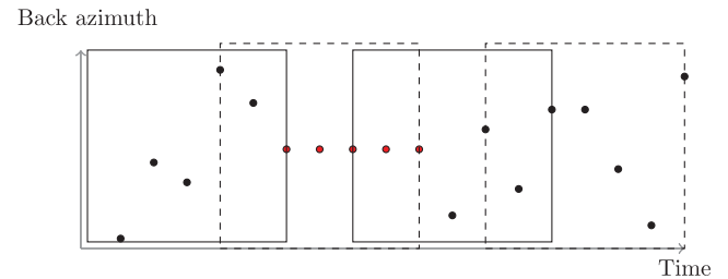
Figure 1. The HW as a sliding window over the beam-forming results. The black dots are due to incoherent noise, and they are therefore randomly distributed. The red dots result from a coherent signal with a constant BA.
