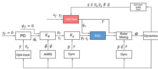
(a) The control structure of G&CNet. A PD controller and an INDI controller are used to keep the quadrotor at y = 0m and \psi = 0^\circ .
