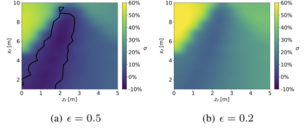
Fig. 4. Comparison of arrival time between DiffG&C and G&CNet. Despite power optimality being weighted equally to time optimality, G&CNet( \epsilon = 0.5 ) can, in most cases, steer the drone to the target points in less time than DiffG&C (the black line shows the region border where G&CNet outperforms DiffG&C). On the other hand, G&CNet( \epsilon = 0.2 ) is always faster than DiffG&C.
