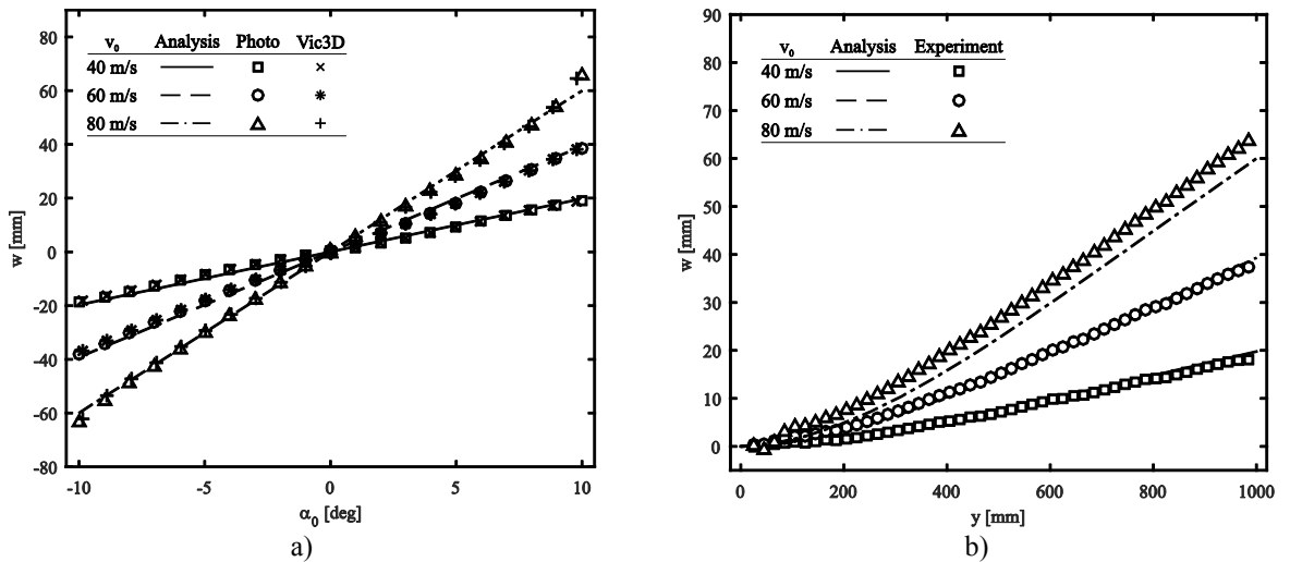
Figure 11: a) CS out-of-plane tip deflection at \alpha_0 and b) CS out-of-plane deflection of the quarter-chord line at \alpha_0 = 10^\circ
