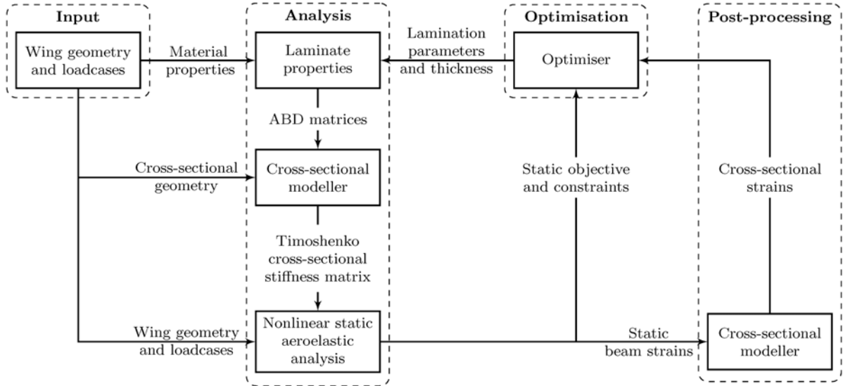
Figure 1: Static aeroelastic analysis module
