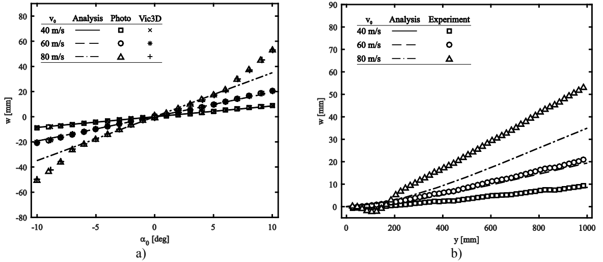
Figure 10: a) QI out-of-plane tip deflection at \alpha_0 and b) QI out-of-plane deflection of the quarter-chord line at \alpha_0 = 10^\circ
