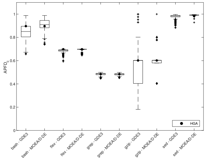
Fig. 8. APFD_c scores achieved by GDE3 (boxplots), MOEA/D-DE (boxplots), and HGA ( \bullet ) on the five-criteria (four-objective) formulation of TCP problem.
