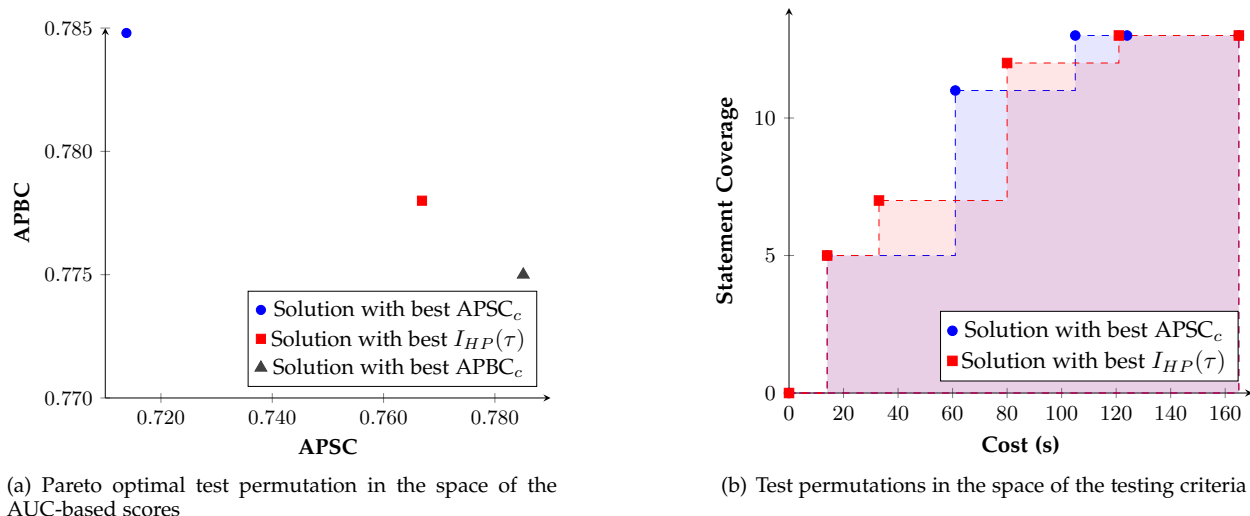
Fig. 3. Comparison of the Pareto optimal solutions (test prioritizations) for the test suite in Table 1 and the solution with the best I_{HP} score.
