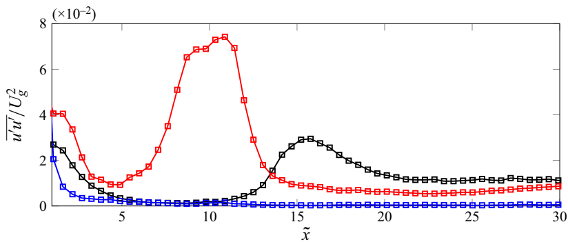
Figure 16. Profiles of \bar{u'u'}/U_g^2 at \tilde{y} = 0 for different values of the gas Reynolds number, for cases REF (black curve), G2 (red curve) and G4 (blue curve) of table 3.
