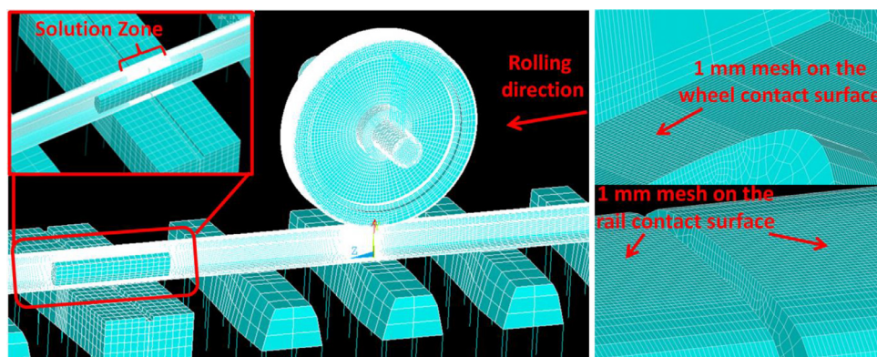
(a) Wheel-IRJ interaction model
