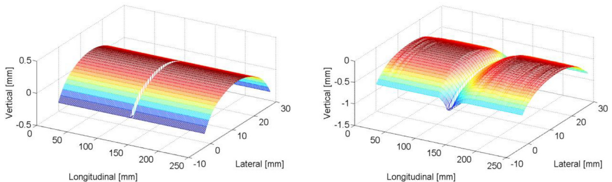
(a) Nominal geometry at the IRJ
