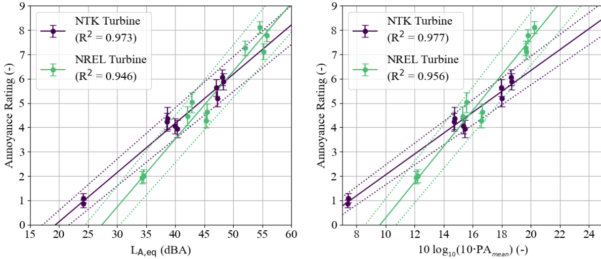
Figure 9 Correlation between the mean annoyance ratings reported in the listening experiments and L_{A,eq} (left) and PA (right, in logarithmic scale). Data points show the mean annoyance ratings and their standard errors. The dotted lines show the standard errors of the Least-Squares fit curves.
