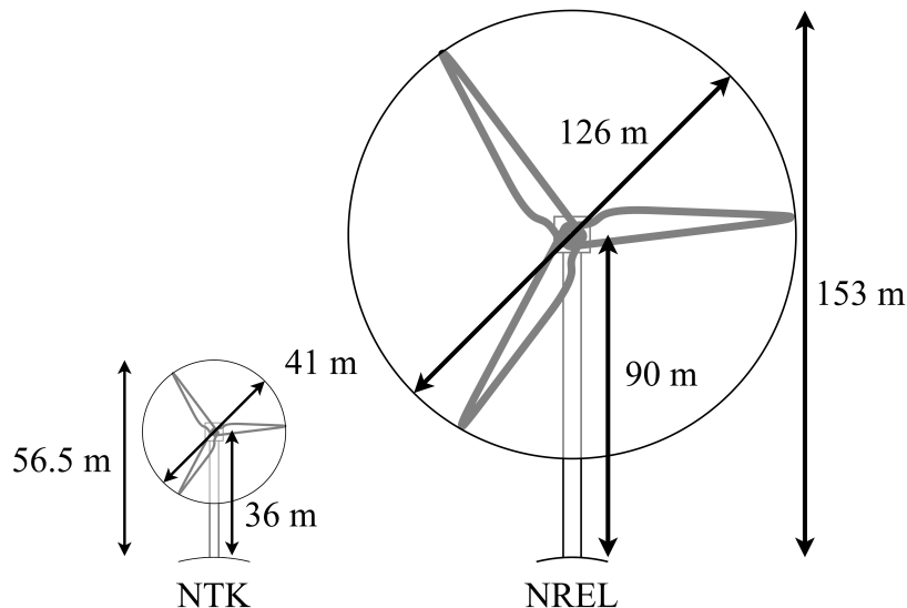
Figure 1 Size comparison of the NTK and NREL wind turbine models used in this work.
