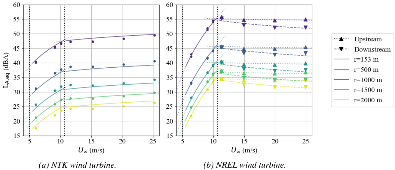
Figure 3 A-weighted equivalent sound pressure levels of the auralisations and the least-squares model curves.
