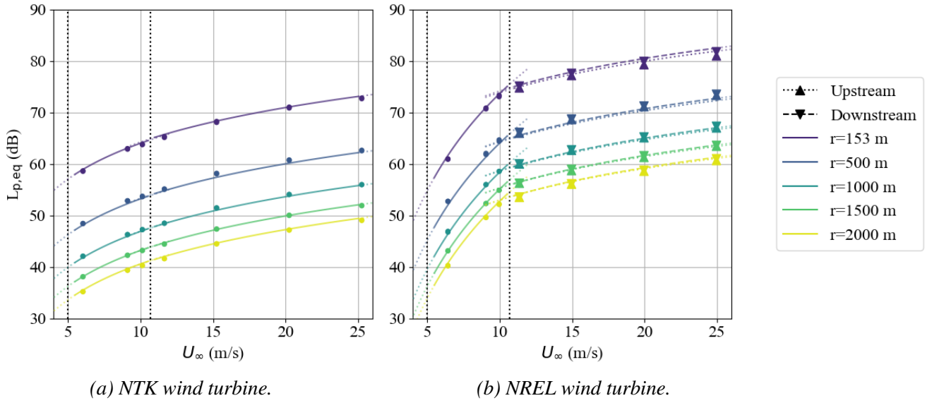
Figure 2 Equivalent sound pressure levels of the auralisations and the least-squares model curves.
