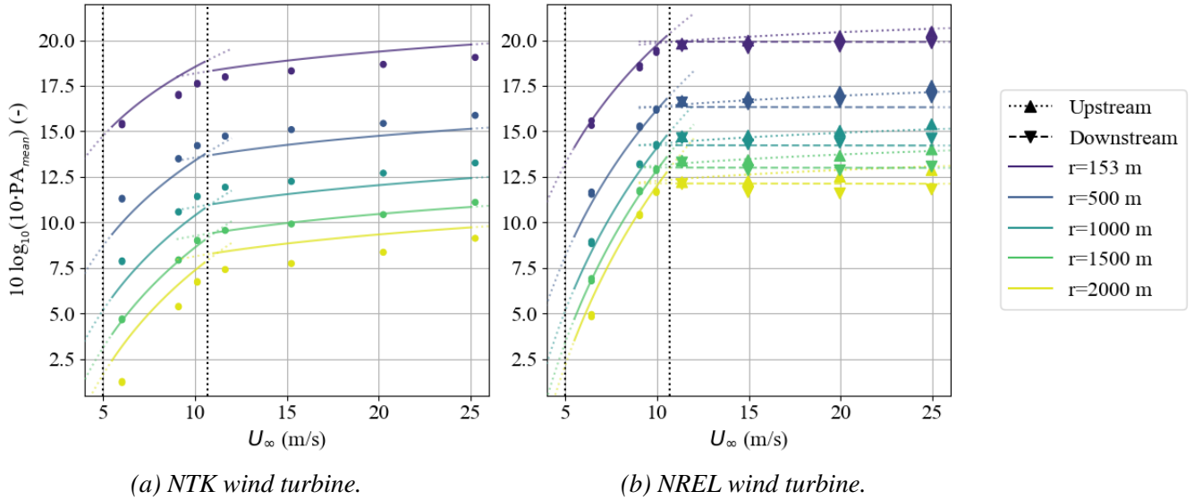
Figure 5 Mean Psychoacoustic Annoyance (PA) of the auralisation results and the least-squares model curves.
