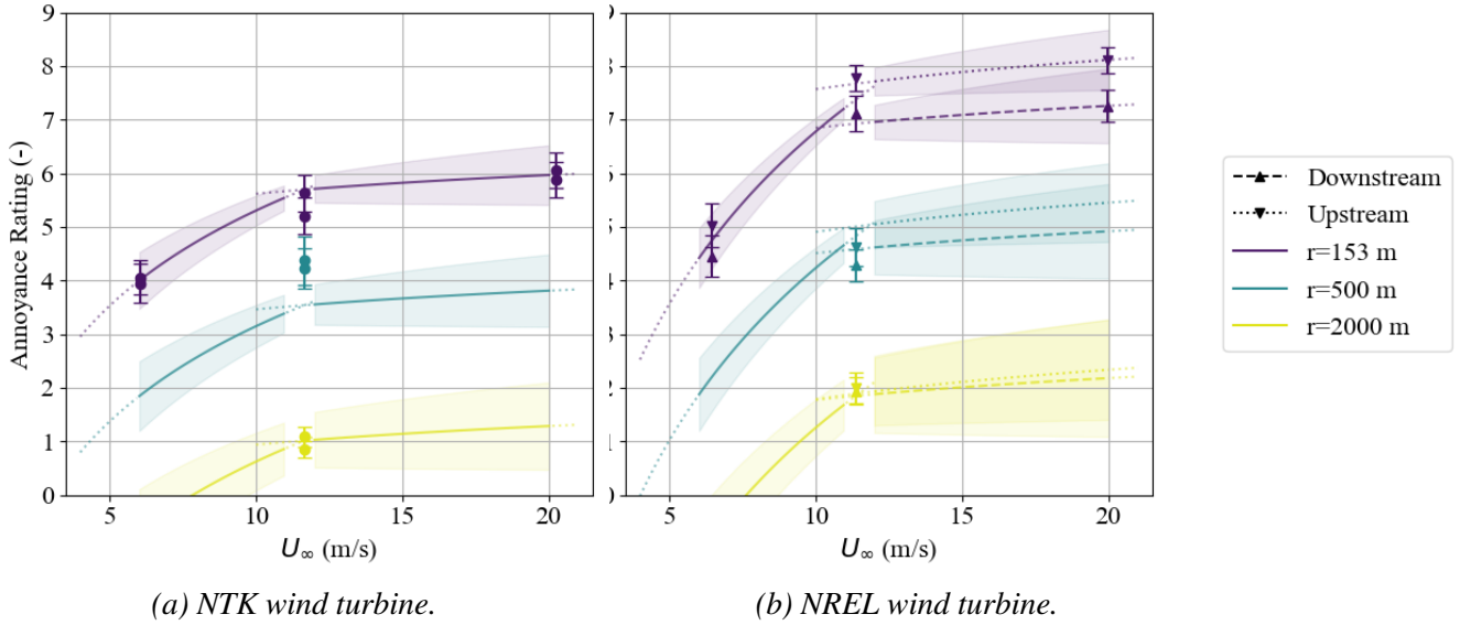
Figure 8 Listening experiment mean annoyance ratings and their standard errors, and least-squares fit curves for the NTK (left) and NREL (right) wind turbines. Shaded areas indicate the confidence intervals of the least-squares models.
