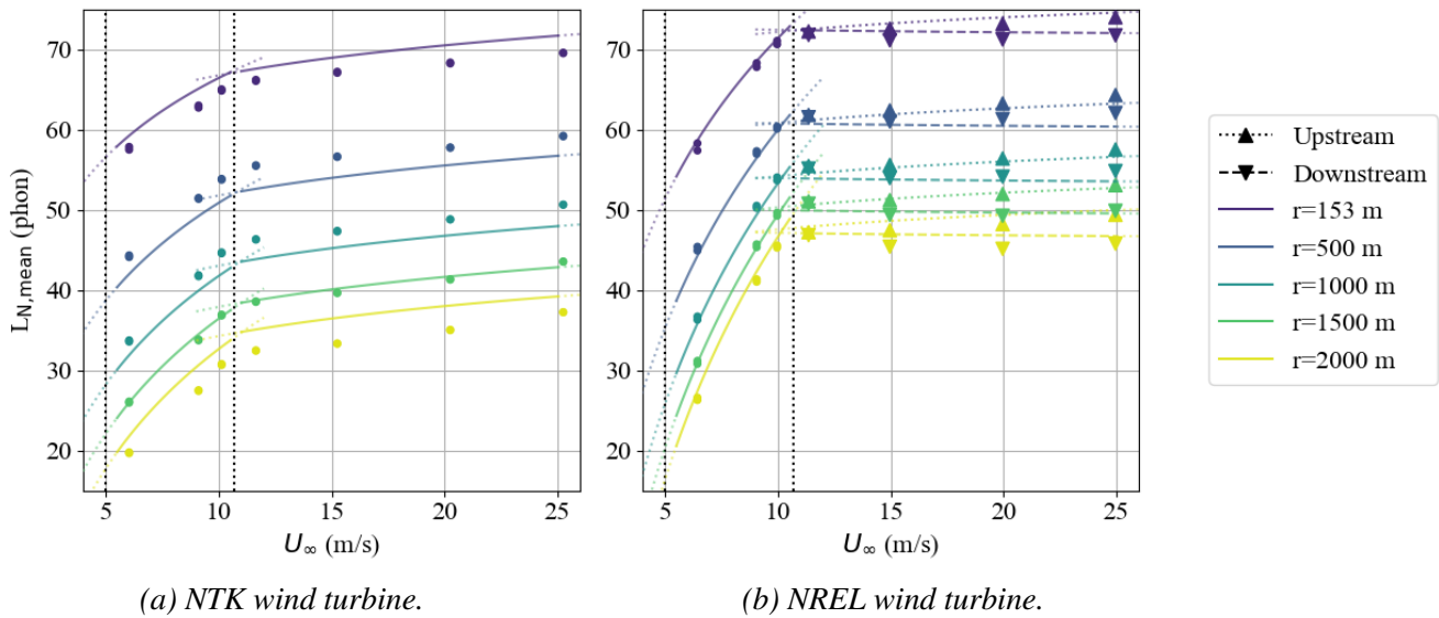
Figure 4 Mean loudness level of the auralisation results and the least-squares model curves.
