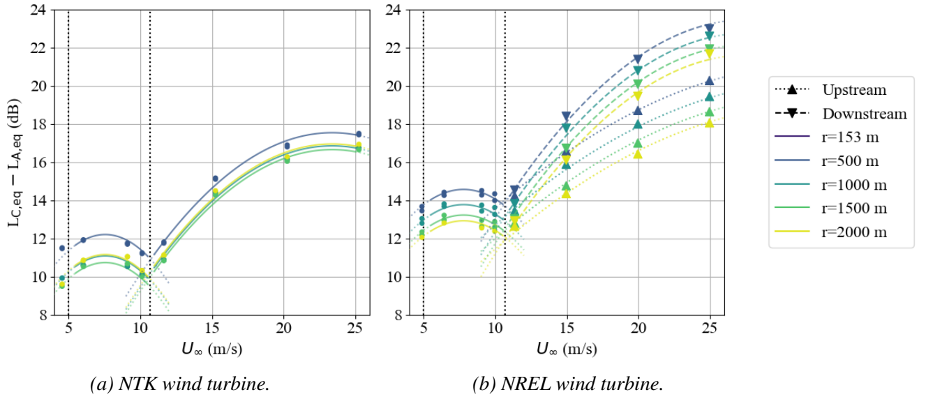
Figure 6 Difference between C- and A-weighted sound pressure levels of the auralisation results, as a measure of low frequency noise content, and the least-squares model curves.
