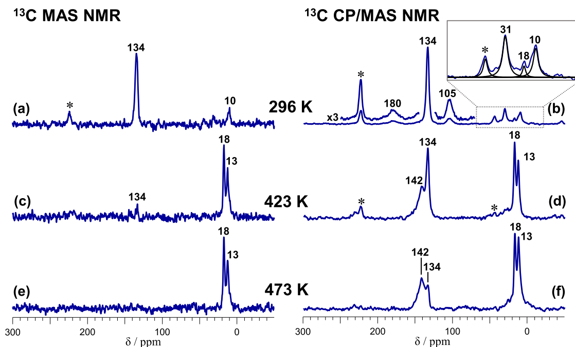
Figure 1. ^{13}C MAS NMR (a,c,e) and ^{13}C CP/MAS NMR (b,d,f) spectra of ethene- ^{13}C_1 adsorbed on Zn^{2+}/ZSM-5 zeolite. The sample was successively heated ex situ for 5 min at 296 (a,b), 423 (c,d), and 473 K (e,f). Asterisks (*) denote spinning sidebands.
