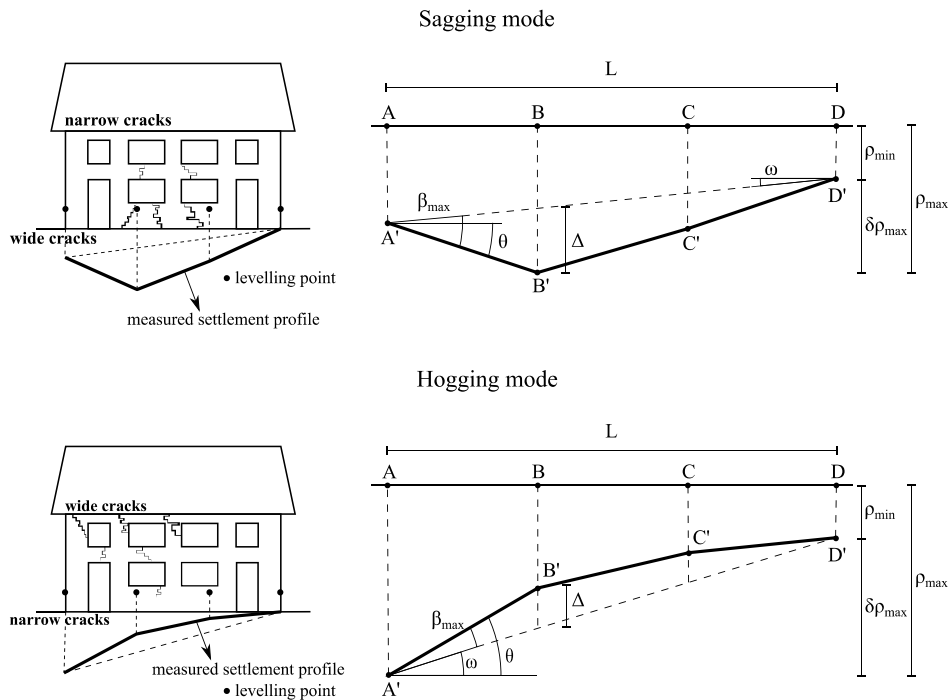
Fig. 3. Typical building damage for sagging and hogging profiles and the definitions of the settlement parameters: maximum settlement \rho_{\max} , minimum settlement \rho_{\min} , differential settlement \delta\rho_{\max} , rotation \theta , relative rotation (or angular distortion) \beta , deflection \Delta , deflection ratio \Delta/L and tilt \omega .
