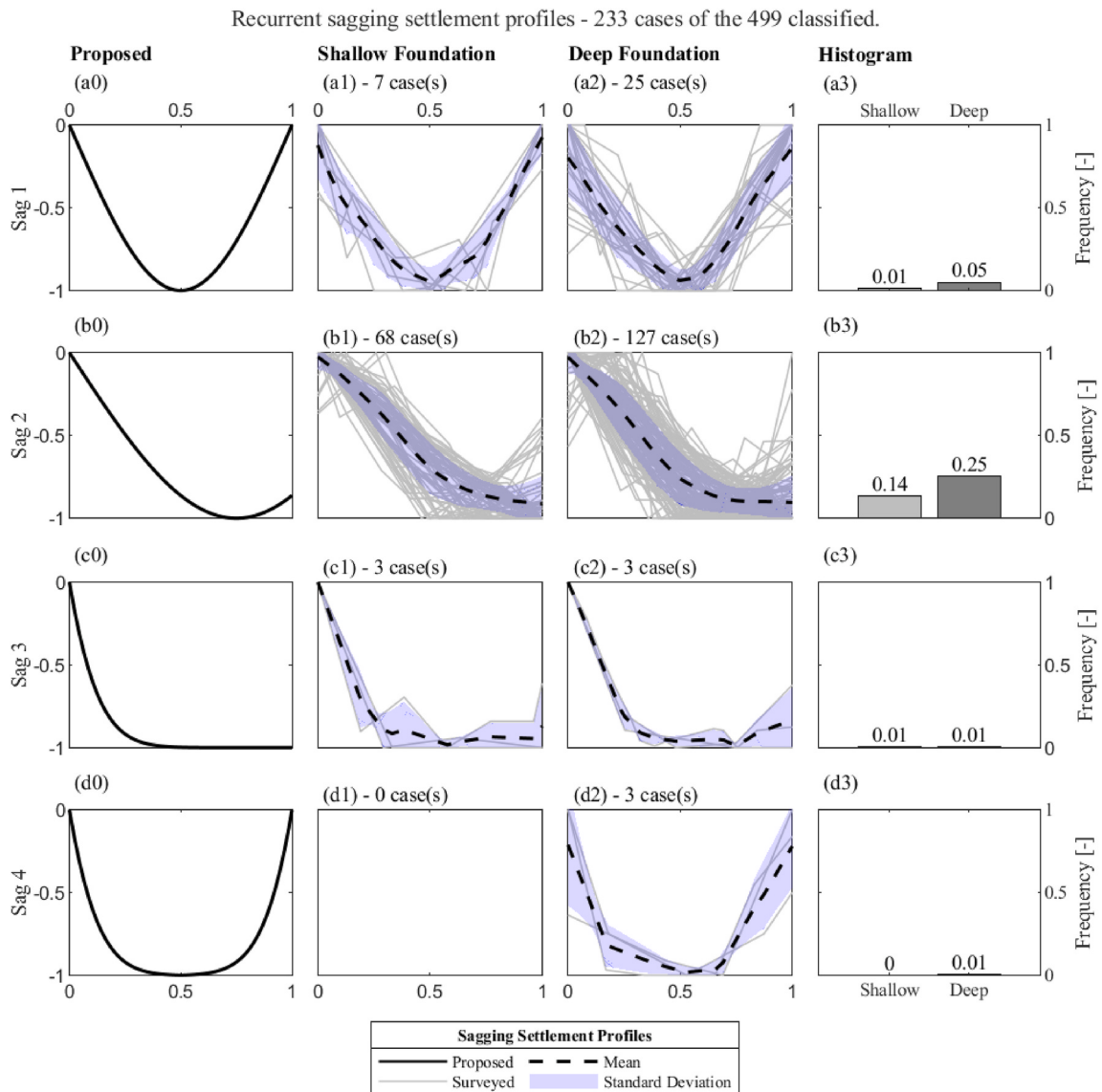
Fig. 9. Nondimensional sagging settlement profiles of the considered surveyed buildings: from (a0) to (d0) Proposed settlement profiles; Settlement profile for: from (a1) to (d1) for buildings on shallow foundations, and from (a2) to (d2) for buildings on deep foundations. The number of cases for each foundation system is indicated on top of each bin from (a3) to (d3).
