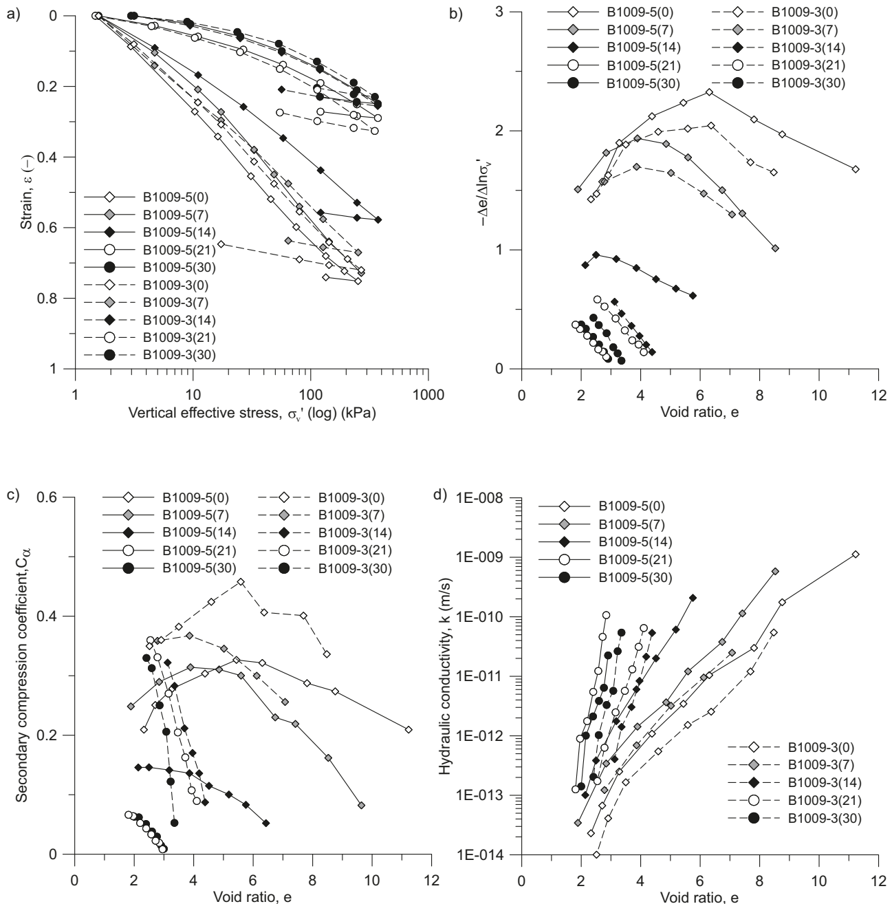
Fig. 10. Effect of organic content on (a) compression curves; (b) -\Delta e/\Delta \log \sigma'_v ; (c) C_\alpha ; (d) k .
