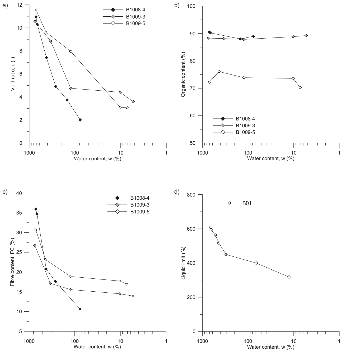
Fig. 1. Effect of drying on (a) void ratio; (b) organic content; (c) fibre content; (d) liquid limit.
