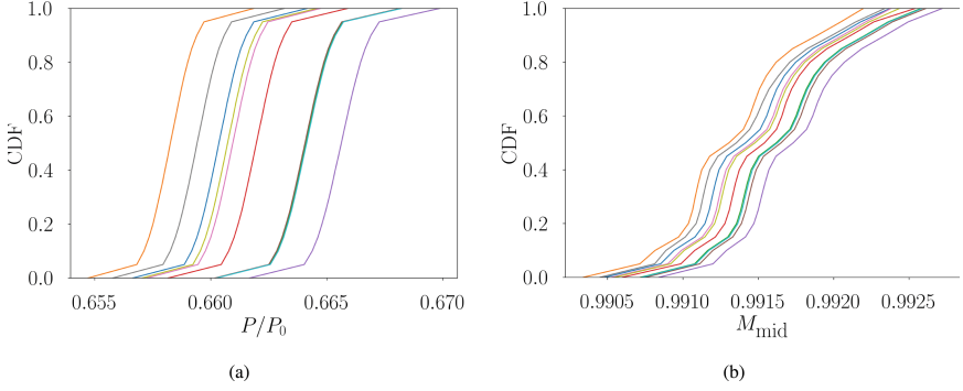
Fig. 2. CDFs corresponding to [518.72 K, 19.1 bar] — blue —, [518.81 K, 19.33 bar] — orange —, [519.82 K, 18.92 bar] — green —, [520.53 K, 19.24 bar] — red —, [521.18 K, 19.01 bar] — purple —, [521.41 K, 19.19 bar] — brown —, [519.29 K, 19.13 bar] — pink —, [519.63 K, 19.35 bar] — grey —, [518.81 K, 19.42 bar] — yellow —, [520.14 K, 18.97 bar] — teal —. (a) Family of CDFs for the pressure value at the nozzle wall at x = 0.0424 m from the inlet. (b) Family of CDFs for the centerline Mach number at x = 0.0424 m from the inlet.
