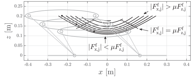
Fig. 4. Snapshots and trajectories of the trunk corresponding to autonomous orbits on the Eigenmanifold presented in Fig. 3 for a range of energy levels. This mode does not excite the rotation of the trunk, and the resulting swinging motion is exploited to build quasi-passive gaits. If we remove the constraint at the feet, the dotted lines delineate the border between the feasible and unfeasible motion (since a foot either loses contact or slides for |F_x^f| > \mu F_z^f , see footnote 3 below).
