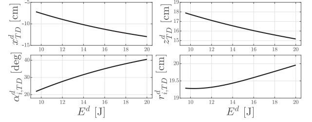
Fig. 6. State at touchdown (top plots) in function of the mechanical energy using modal information, with corresponding attack angles and leg lengths (bottom plots). To connect the stance phase modes for different speeds (i.e., different energy levels), a proper attack configuration is required.
