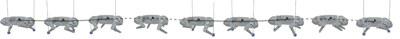
Fig. 12. Snapshots of the robot performing trotting in Gazebo. The blue dots denote contacts between the feet and the ground.
