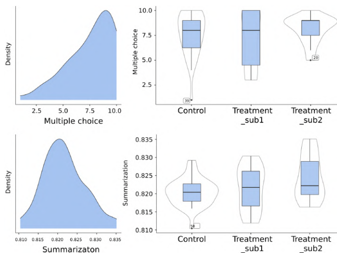
Figure 8.7: Knowledge gain distributions for multiple choice and summarization tasks in 3-condition comparison with control, Treatment_sub1, and Treatment_sub2 groups.
