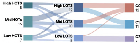
Figure 4.7: The usage of high, mid, and low ranges of HOTS & LOTS and their relations to clusters derived from k-means clustering.
