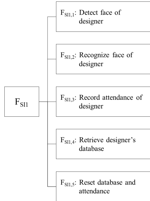
Figure 4.10. High-level functional decomposition of F_{SI1}
