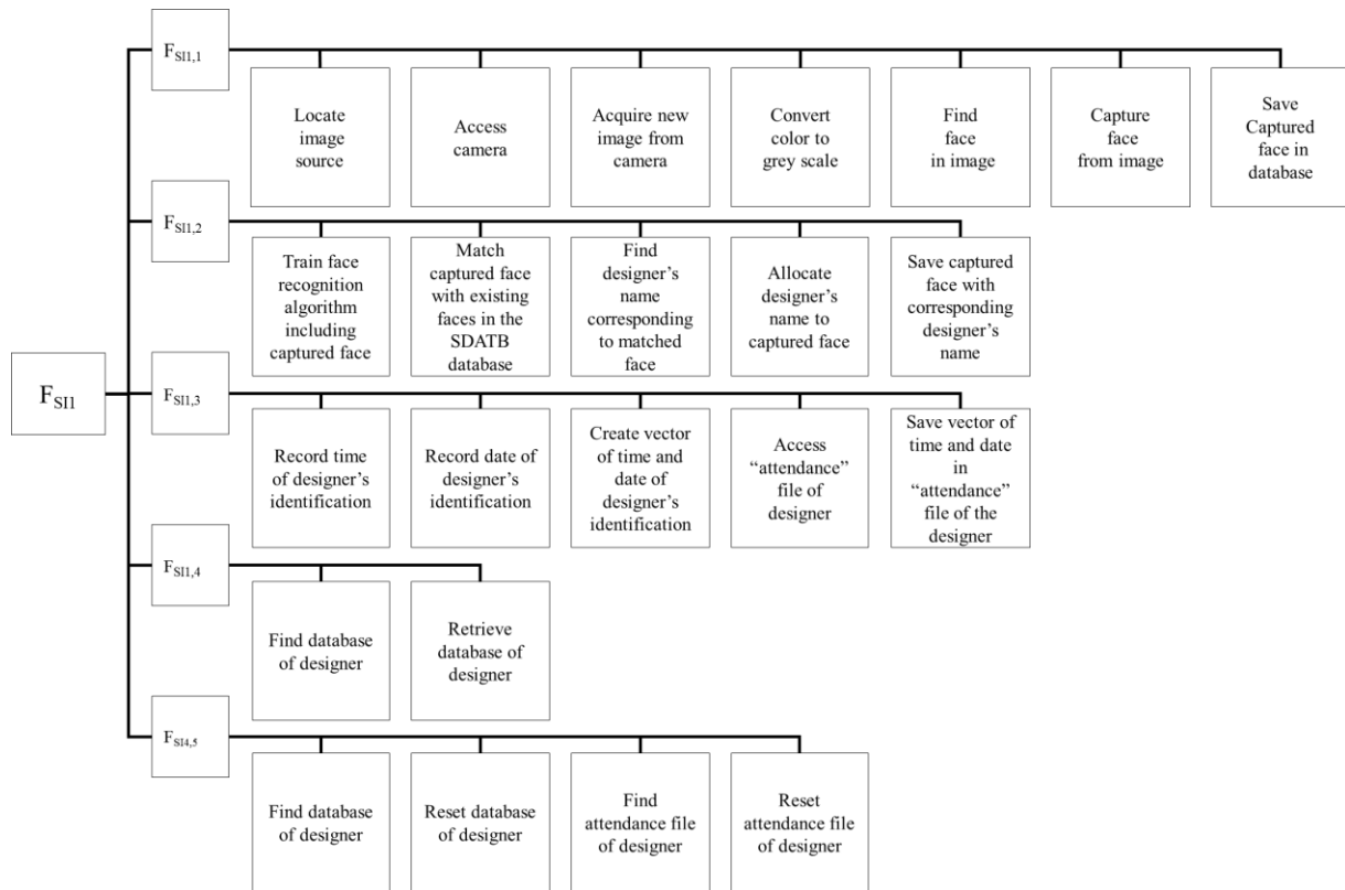
Figure 4.11. Low-level functional decomposition of F_{S11}
