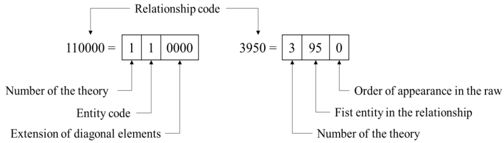
Figure 3.13. Example of coding used for fused theories
