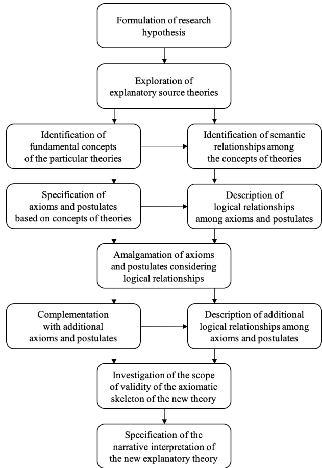
Figure 3.5. The logic of axiomatic theory fusion
