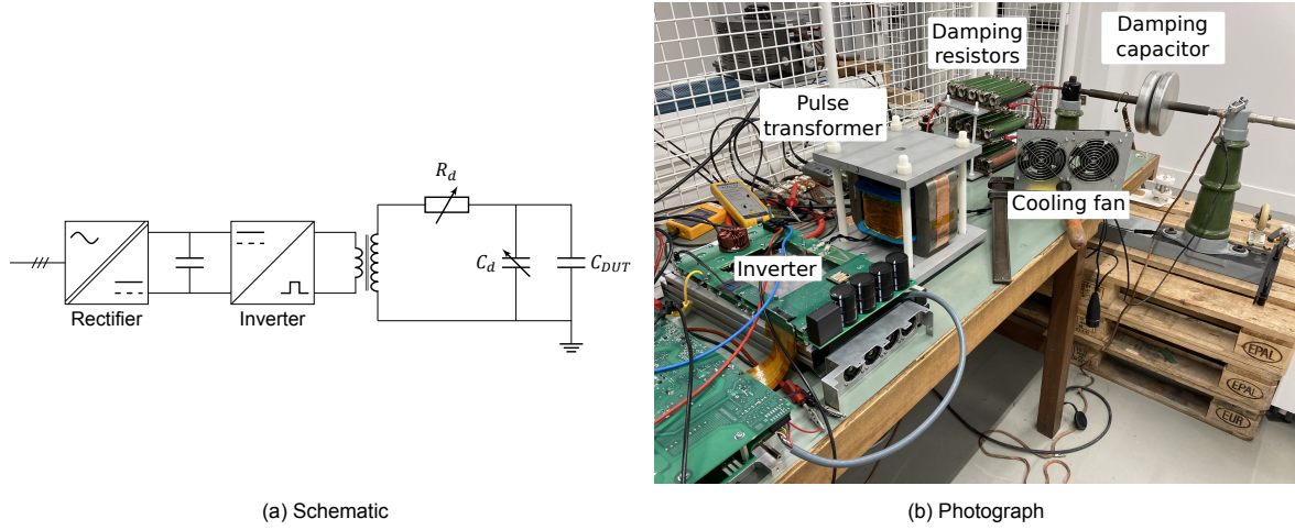
Figure 3.5: Test Setup for square-wave voltage.
