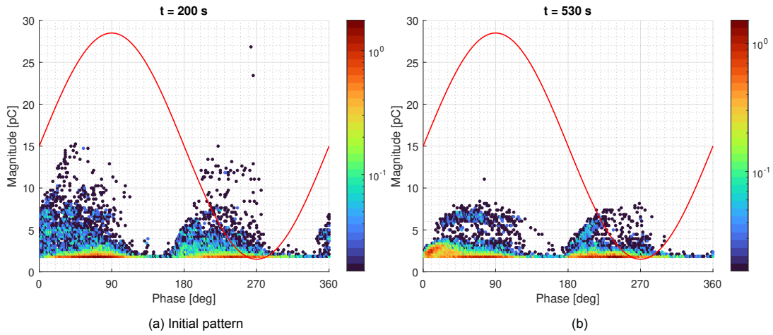
Figure D.6: PRPD of Sample B at 5.2 kV rms .
