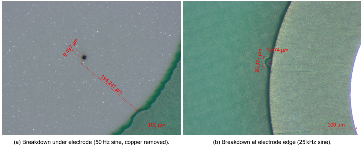
Figure 4.9: Micrographs of broken samples.
