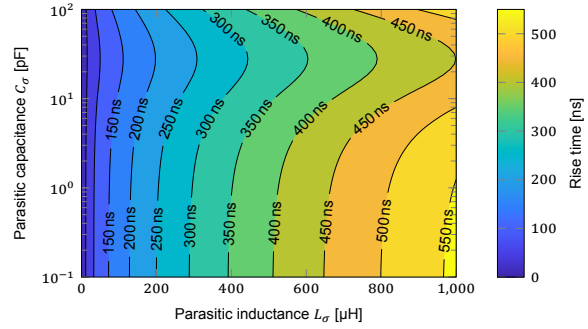
(b) Rise time vs parasitic components (with C_{DUT} = 68 \text{ pF} and \zeta = 1/\sqrt{2} ).
