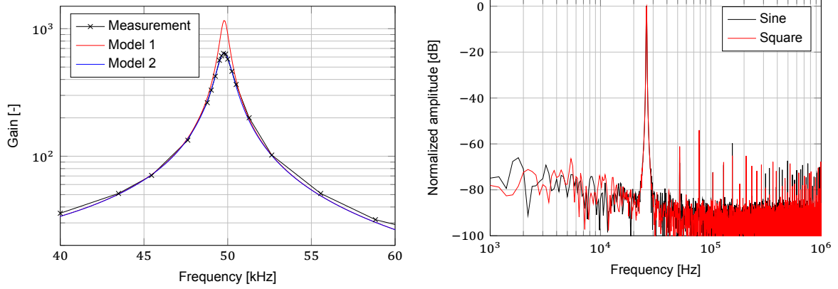
(a) Transfer function of RT2 ( C_{DUT} = 90 pF, \tan \delta = 300 \times 10^{-4} @ 50 kHz and an additional C_{res} = 200 pF with no dielectric loss).
