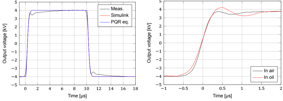
(a) Comparison of pulse response simulations and measurements with f_s = 50 \text{ kHz} , C_{DUT} = 68 \text{ pF} and R_d = 4.6 \text{ k}\Omega . (b) Pulse response comparison with and without transformer oil.
