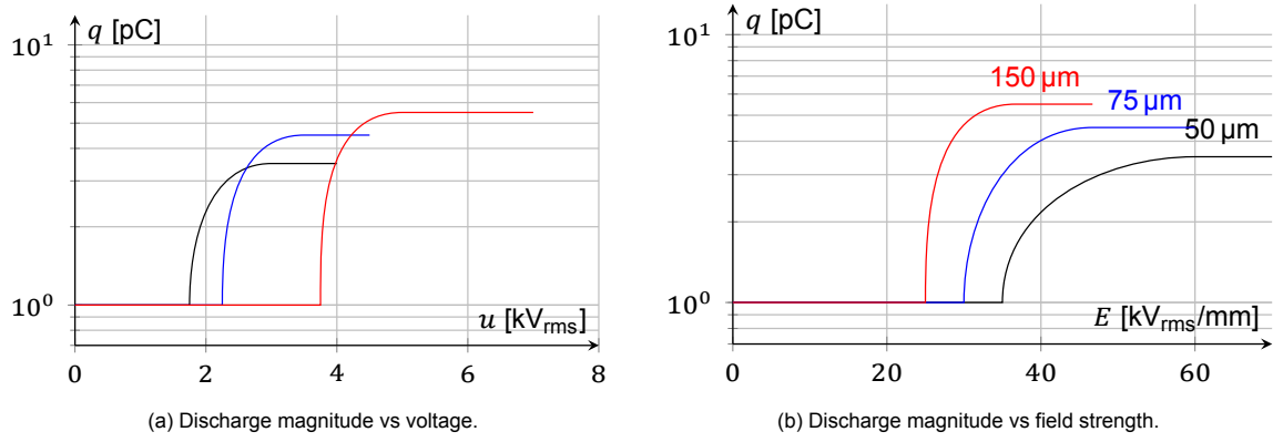
Figure 4.15: Internal discharge inception.
