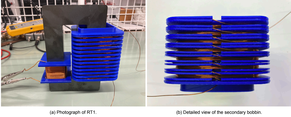
Figure C.4: Photographs showing the split winding configuration and bobbin designs.
