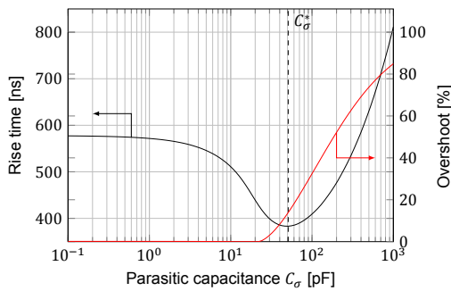
(a) Rise time and overshoot vs C_\sigma for L_\sigma = 440 \mu\text{H} , C_{eq} = 90 \text{ pF} , and R_d = 4 \text{ k}\Omega .
