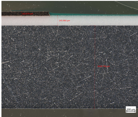
(a) 2 mm aluminium base, 230 \mu\text{m} dielectric, 3 oz copper.
