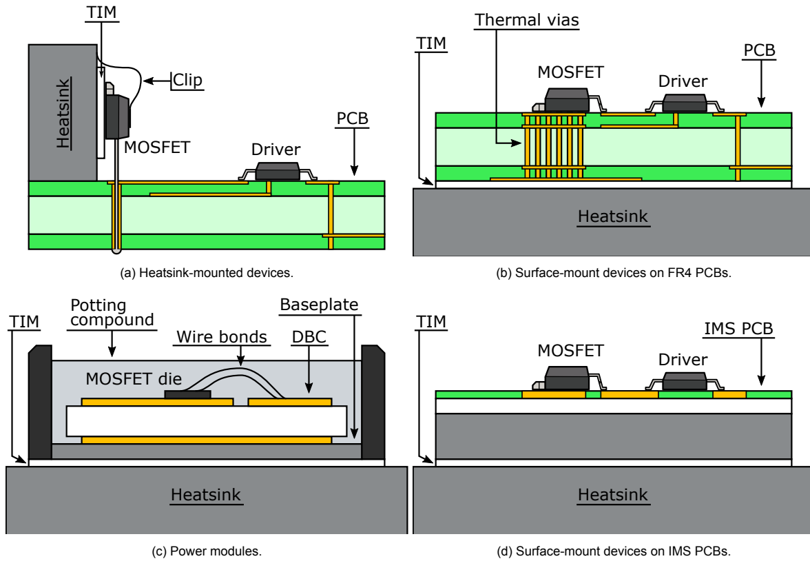
Figure 1.1: Cooling solutions.
