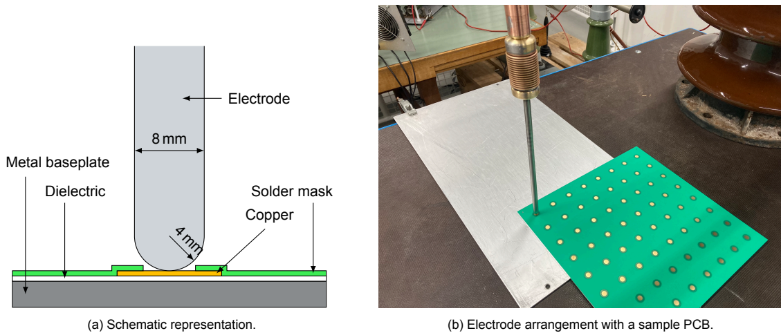
Figure 3.3: Electrode arrangement for testing circular samples.
