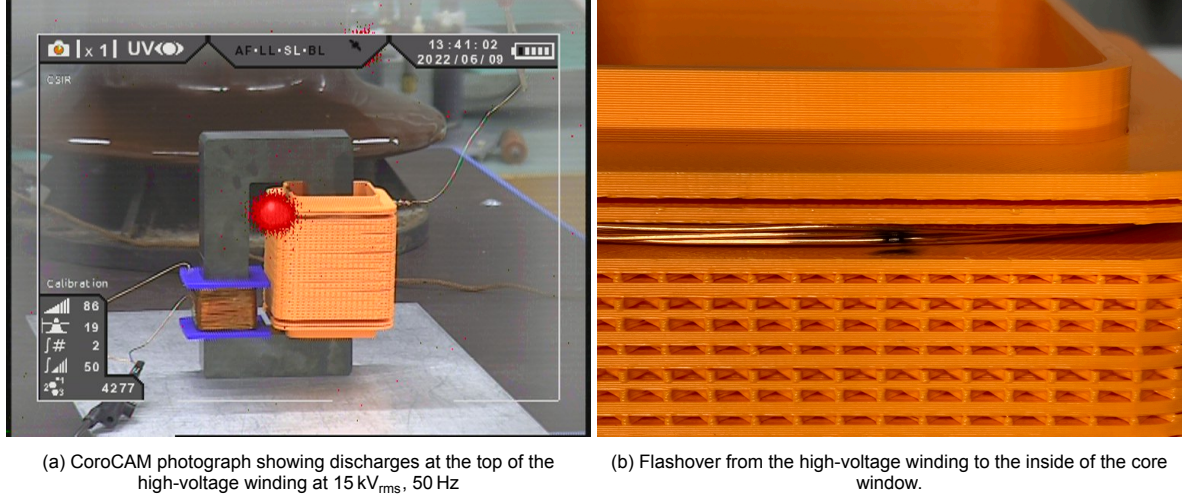
Figure C.7: Photographs of the withstand test results.
