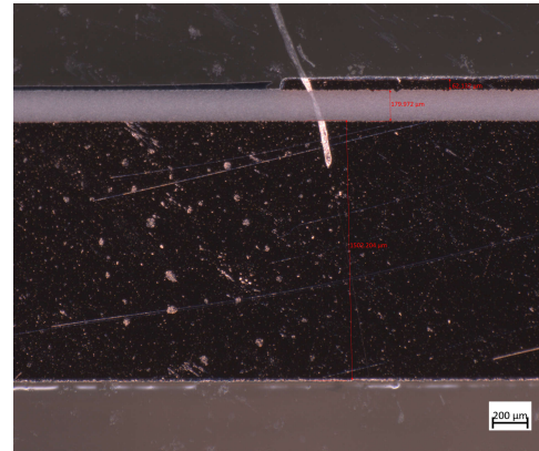
(b) 1.5 mm copper base, 180 \mu\text{m} dielectric, 2 oz copper.
