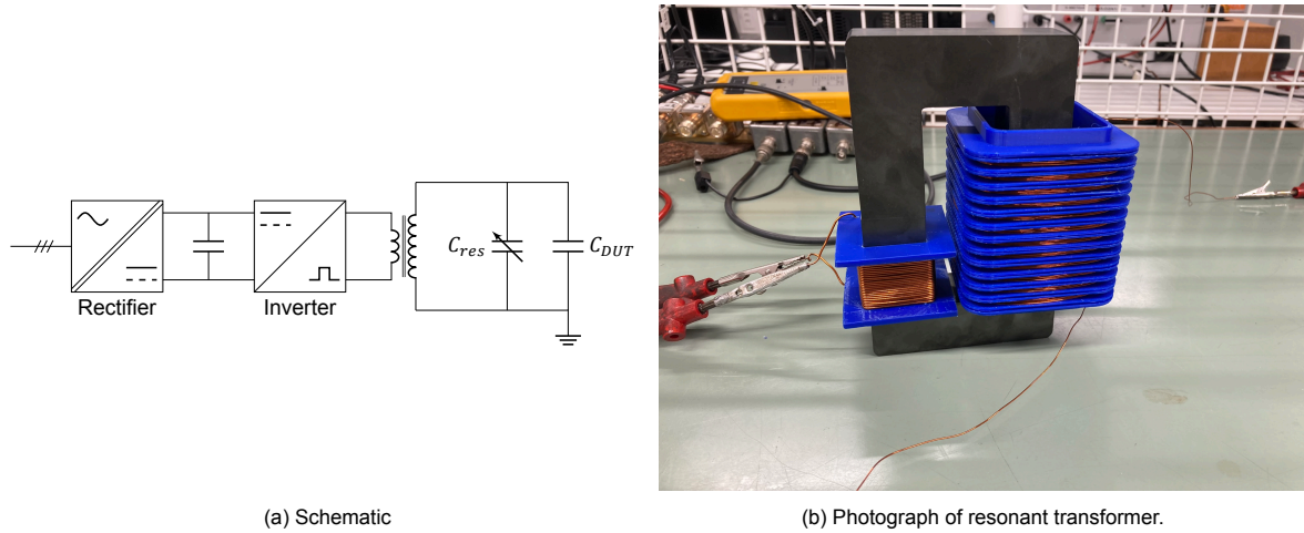
Figure 3.6: Test setup for HF sinusoidal voltage.
