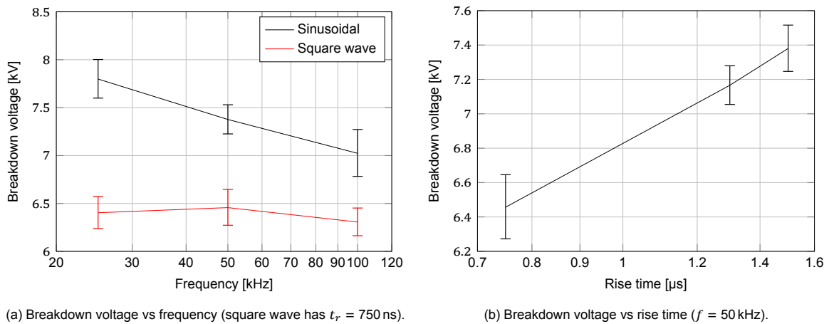
Figure 4.5: Comparison of sinusoidal and square wave voltage.
