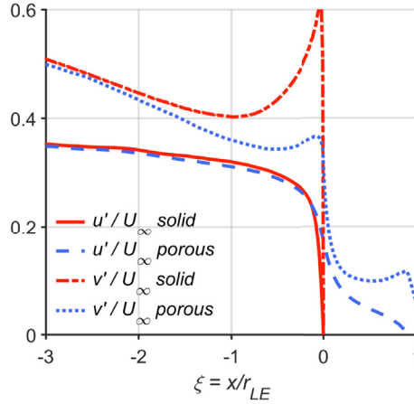
Fig. 14. Turbulence intensity for the solid (red lines) and the porous airfoil (blue lines) extracted by the LES along the stagnation streamline. The u' - and the v' -component are made dimensionless by the free-stream velocity, U_\infty . (For interpretation of the references to colour in this figure legend, the reader is referred to the Web version of this article.)
