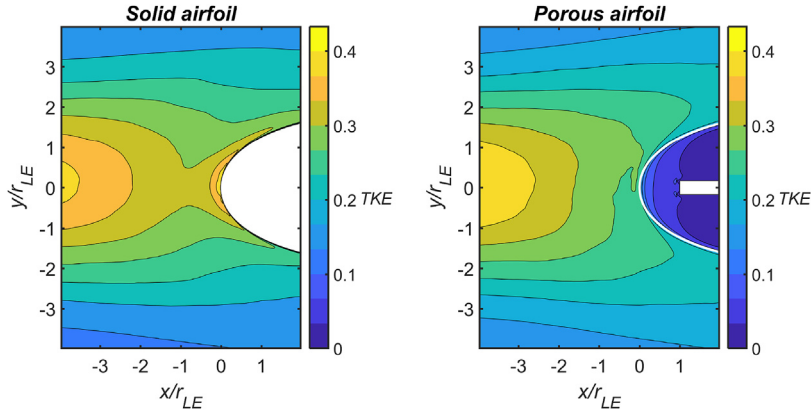
Fig. 15. Turbulent kinetic energy for the solid (on the left) and the porous airfoil (on the right) in the stagnation region extracted by the LES and made dimensionless by the free-stream velocity, U_\infty .
