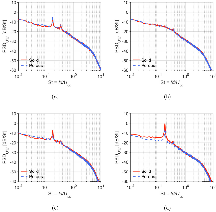
Fig. 16. Velocity fluctuations PSD for the solid (solid red line) and the porous case (dashed blue line) computed from the hot-wire measurements at (a) \xi = x/r_{LE} = -6.7 , (b) \xi = -1 , (c) \xi = -0.5 , and (d) \xi = -0.05 with a reference of 1 \text{ m}^2\text{s}^{-2} . (For interpretation of the references to colour in this figure legend, the reader is referred to the Web version of this article.)
