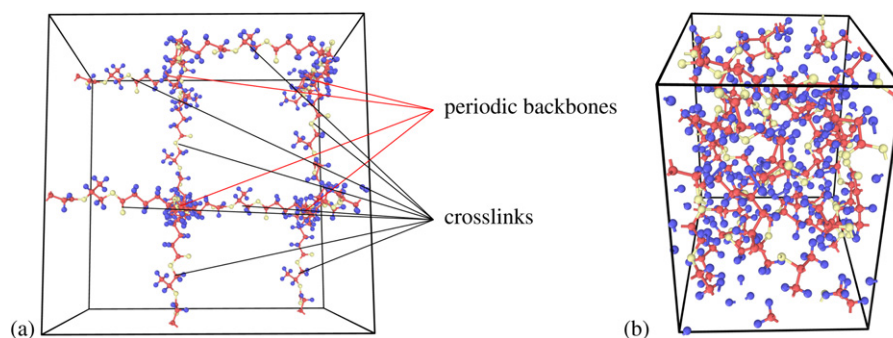
Fig. 2. (a) 0K, 0 atm low density, and (b) 300K, 1atm equilibrated 50 % crosslinked PPGDA polymer 520-atom unit cell (C=red, H=blue, O=yellow).
