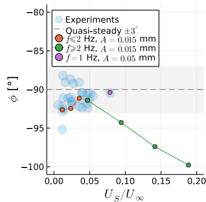
Figure 16. Maximum surge velocity effect on the phase between the rotor position and its thrust.
