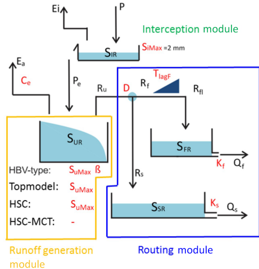
Figure 5. Model structure and free parameters, involving four runoff generation models (HBV-type, TOPMODEL, HSC, and HSC-MCT). HBV-type has S_{uMax} and \beta two free parameters; TOPMODEL and HSC models have S_{uMax} as one free parameter; and the HSC-MCT model does not have a free parameter. In order to simplify calibration process and make fair comparison, the interception storage capacity ( S_{iMax} ) was fixed as 2 mm.
