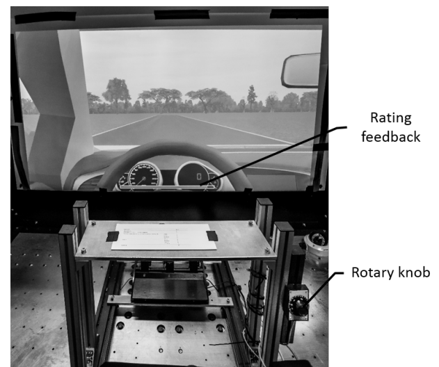
Figure 3: Experiment set up in the hexapod simulator of the MPI for Biological Cybernetics.
