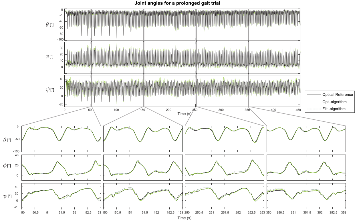
Fig. 8. Resulting 3-D knee joint angles for one subject, obtained from inertial sensor readings with the proposed method for joint kinematic estimation (green: Opt.-algorithm 2, dotted-green: Filt.-algorithm 1) and the optical reference (black) for a prolonged gait trial of 450 seconds. Results are plotted after coordinate frame alignment. Drift is clearly eliminated for the entire duration of the gait trial.
