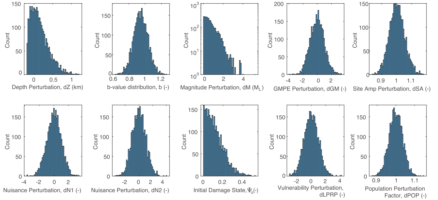
Fig. 4. Perturbed input variables for the Monte Carlo analysis. Ten panels show histograms for each of the perturbed variables of interest: dZ – depth, b – b-value, dM – trailing magnitude, dGM – GMPE variability, dSA – site amplification perturbation factor, dN1 and dN2 – nuisance function variabilities, \Psi_0 – initial damage state, dLPR – vulnerability function variability, and dPOP – population perturbation factor.
