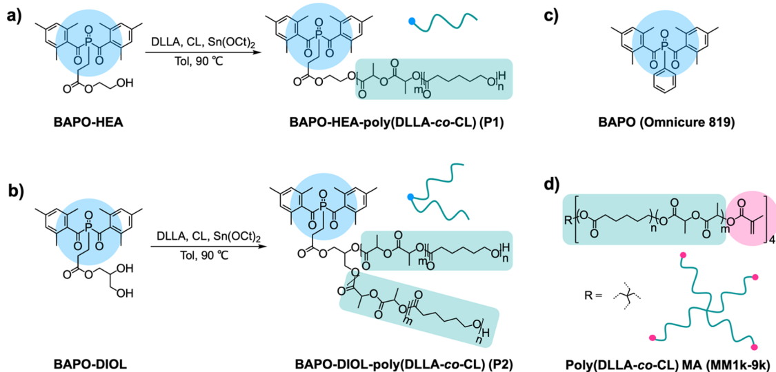
Scheme 1. (a) Synthesis of BAPO-HEA-Poly(DLLA-co-CL) (P1) from BAPO-HEA by Random Copolymerization of DLLA and CL (P1); (b) Synthesis of BAPO-DIOL-Poly(DLLA-co-CL) (P2) from BAPO-DIOL by Random Copolymerization of DLLA and CL; (c) Chemical Structure of a Commercially Available BAPO (Omniscure 819); (d) Chemical Structure of the Macromonomer Poly(DLLA-co-CL) MA (MM1k-9k) Used for 3D Printing
