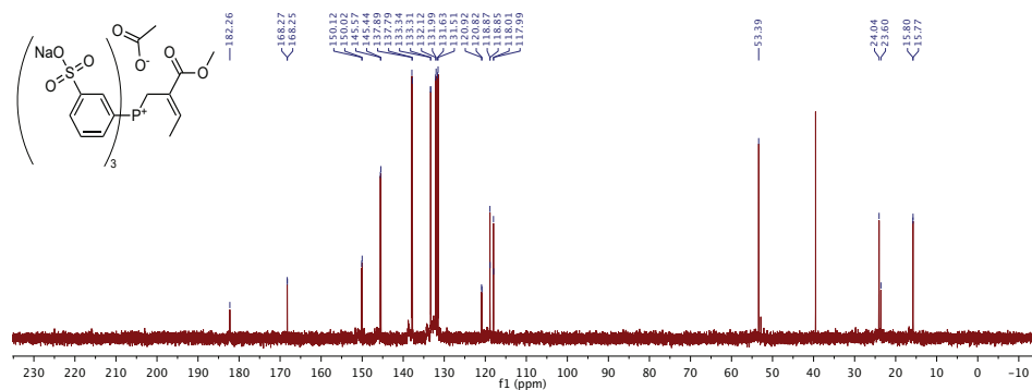
Figure S21: 13 C NMR, compound 1 in D 2 O + 1 μL DMSO.
