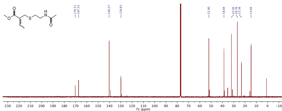
Figure S24: 13 C NMR, compound 2 in CDCl 3 .
