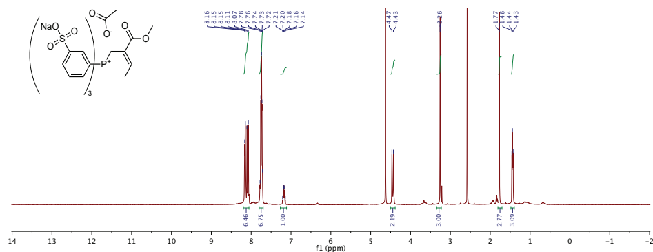
Figure S20: 1 H NMR, compound 1 in D 2 O + 1 μL DMSO.
