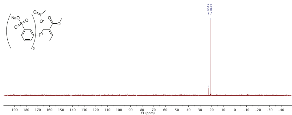
Figure S22: 31 P NMR, compound 1 in D 2 O + 1 μL DMSO.
