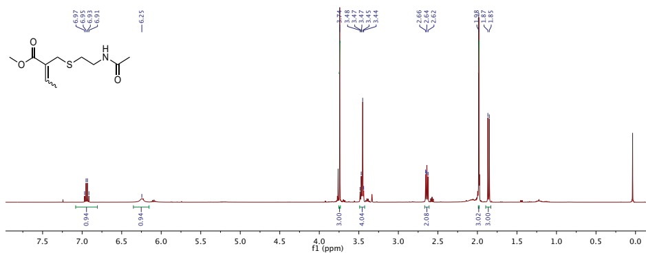
Figure S23: 1 H NMR, compound 2 in CDCl 3 .
