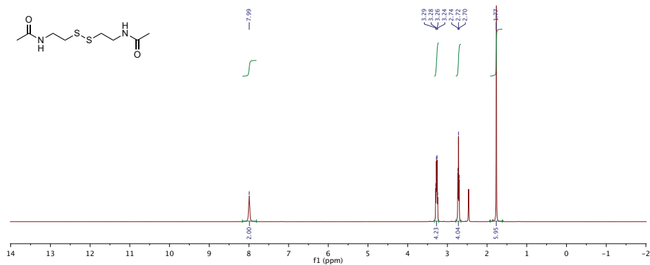
Figure S25: 1 H NMR, compound 3 in DMSO-d 6 .
