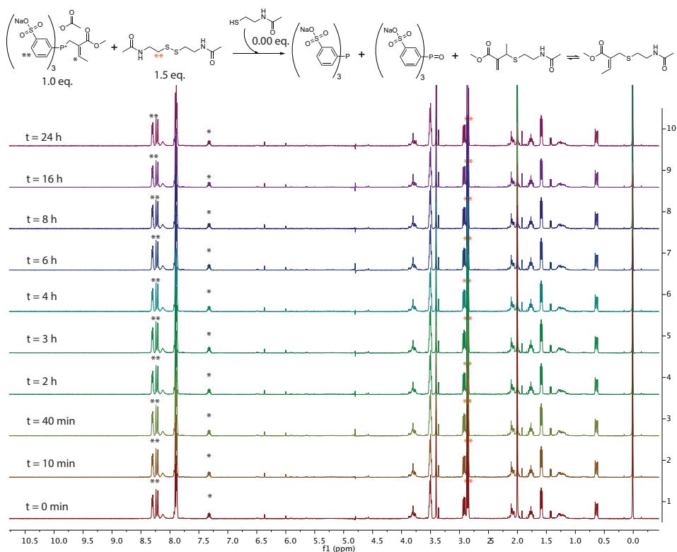
Figure S5: Stability observation of compound 1 and 2 in 1 H NMR at different time points for 24 hours. The reaction was carried out in D 2 O/phosphate buffer mixture 2:8 (0.1 M, pH = 7.6). The spectra were aligned with the D 2 O peak. The peak attributed to ~0.0 ppm corresponds to DSS internal standard.
