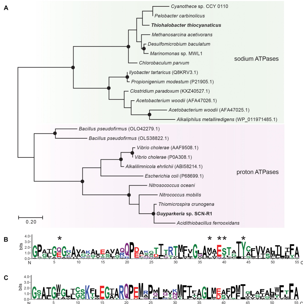
FIGURE 3 | Maximum likelihood tree (A) and sequence logos of sodium (B) and proton-dependent (C) ATP synthases (C-subunit). The sequences of Gyoparkeria sp. SCN-R1 and Thiohalobacter thiocyanaticus HRh1 T are written in bold type. The sodium ligands are indicated with asterisks including the Na + -binding motif ESTxxY (see Mulikdjian et al., 2008). The black dots on the tree indicate bootstrap values between 100 and 75% out of 100 iterations.
