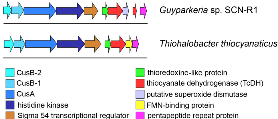
FIGURE 5 | Genome region around TcDH gene in Thiohalobacter thiocyanaticus and Guparkieria SCN-R1. Both organisms contain a number of similar genes around TcDH in the same order (colored arrows). "Blue" genes are likely to be related to a copper transport system (Cus).
