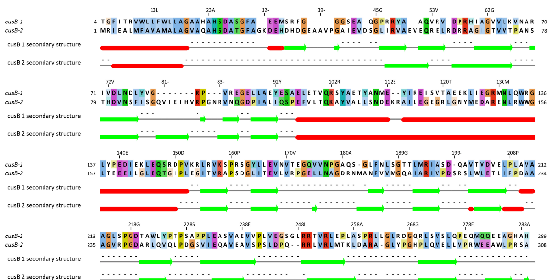
FIGURE 6 | Pairwise alignment of CusB-1 and CusB-2 protein sequences from Thiohalobacter thiocyanaticus performed by Needleman-Wunch algorithm (sequences identity 28%, similarity 43%, and alignment score 186). Secondary structure of each protein was modeled by Jpred 4. Beta-strands and alpha helices are shown by green arrows and red cylinders, respectively.
