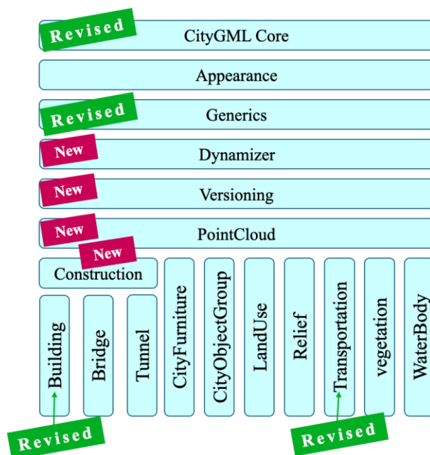
Figure 3. The modules in CityGML 3.0. Image adapted from [10].
