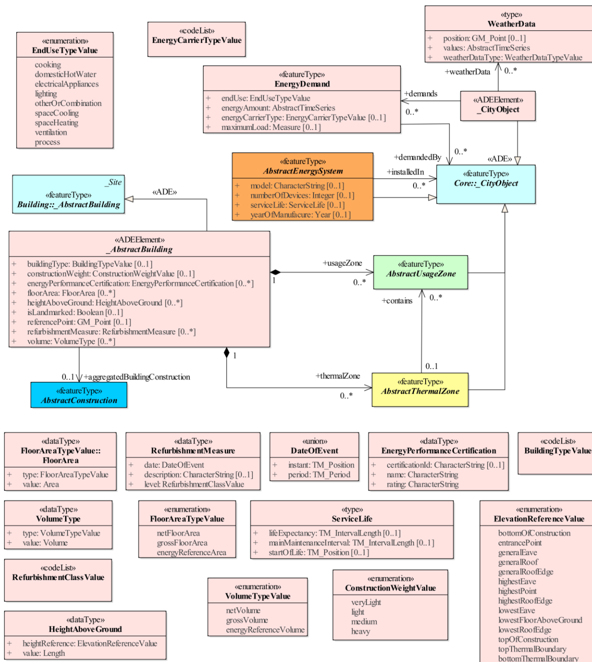
Figure 9. The Core module of the Energy ADE for CityGML 2.0.
