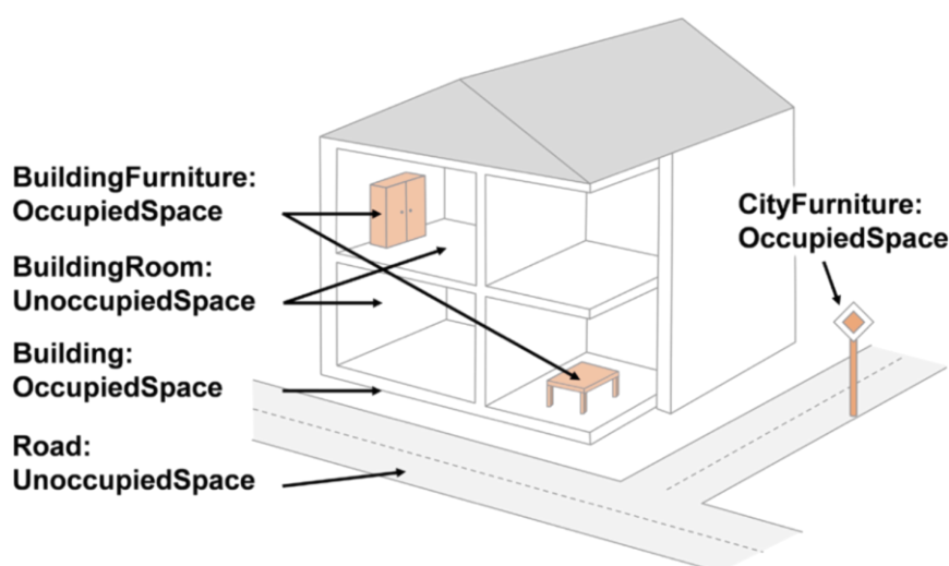
Figure 7. Representation of the classes OccupiedSpace and UnoccupiedSpace using the example of a building. Image taken from [10]
