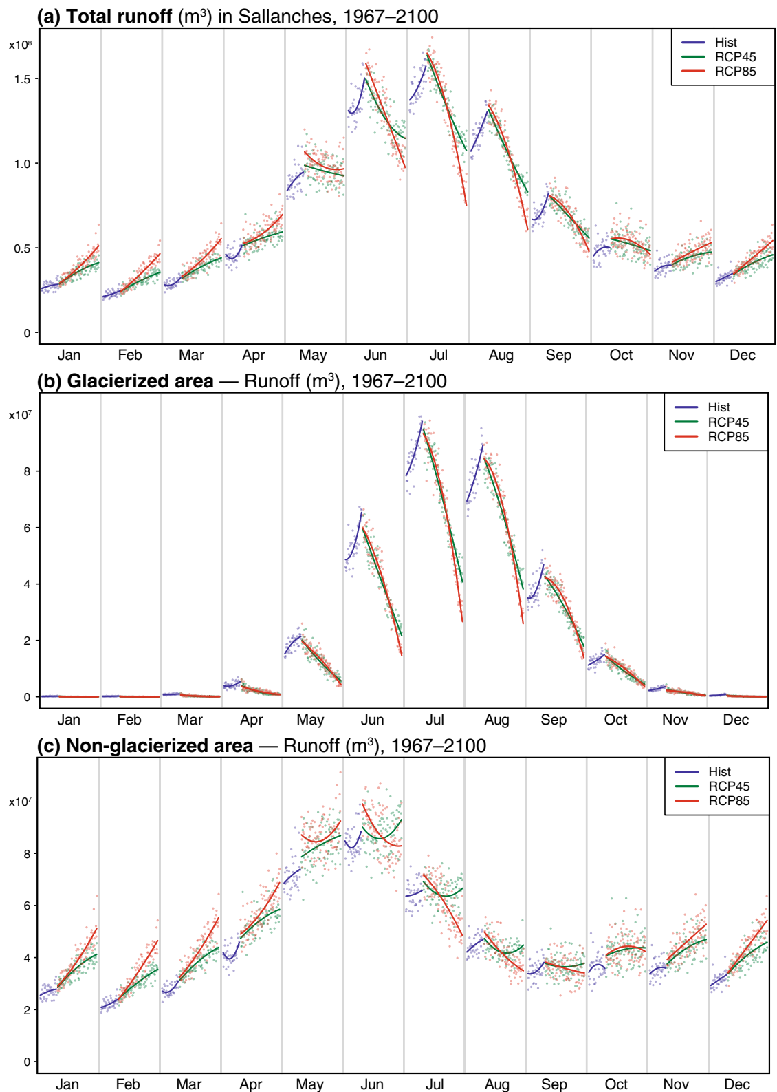
Figure 5. (a) Monthly total runoff in Sallanches ( \text{m}^3 ). (b) Monthly runoff of the ice-covered part of the catchment ( \text{m}^3 ). (c) Monthly runoff of the ice-free part of the catchment ( \text{m}^3 ). Every month's section is a 1967–2100-time series of discharges. Blue colours: historical (Hist) simulations, period 1967–2018. Each point represents the runoff for each year, the curve shows the evolution trend with a quadratic model. Green colours: the same for the RCP4.5 simulations, period 2008–2100. Red colours: the same for the RCP8.5 simulations, period 2008–2100. Graphical representation as in Guichard et al. 51 .
