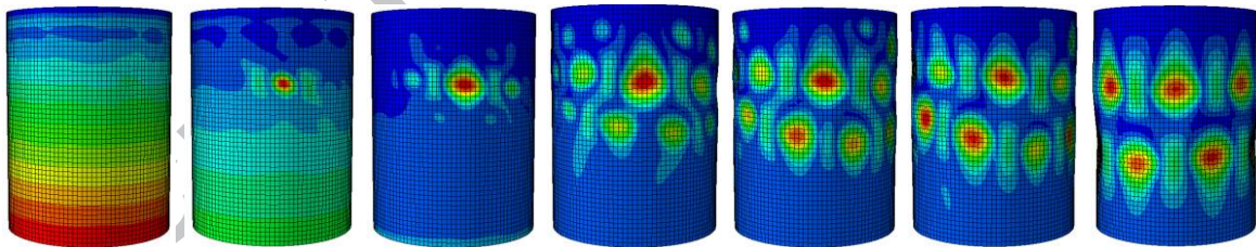
Figure 12. Progression of the buckling shape of the constant-stiffness cylinder
