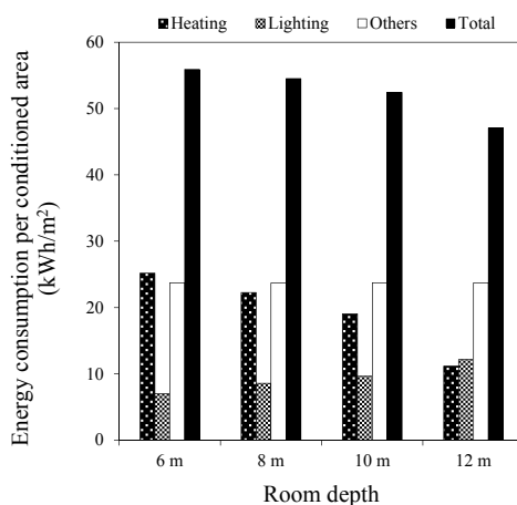
Figure 5. The energy consumption for the south-oriented L shape building with a 40% window to wall ratio (WWR) in terms of room depth.
