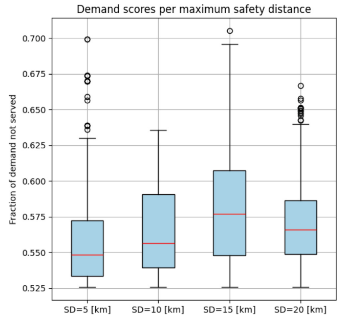
Fig. 16. Boxplot of collected demand objective scores from the Pareto front.
