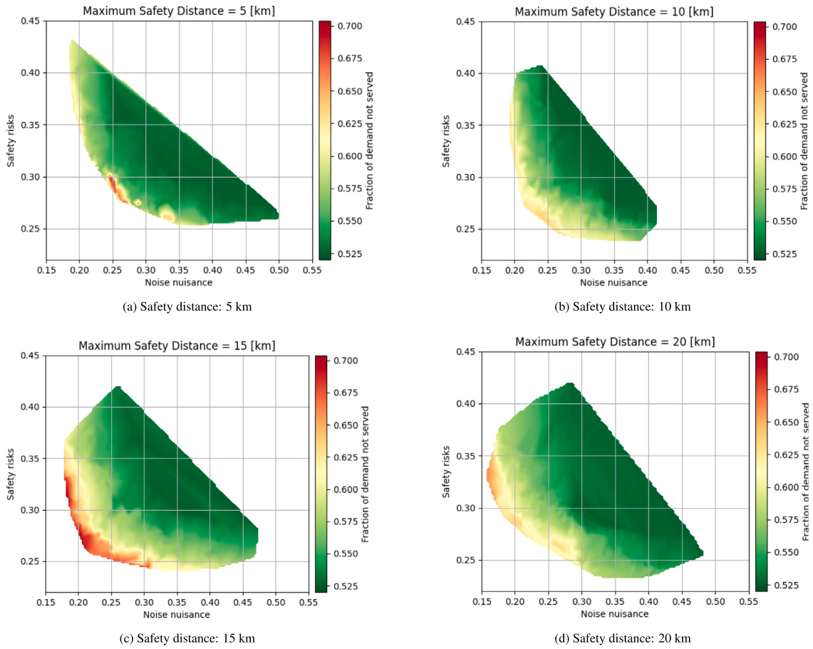
Fig. 14. Pareto front considering a UAM network with different maximum safety distance.
