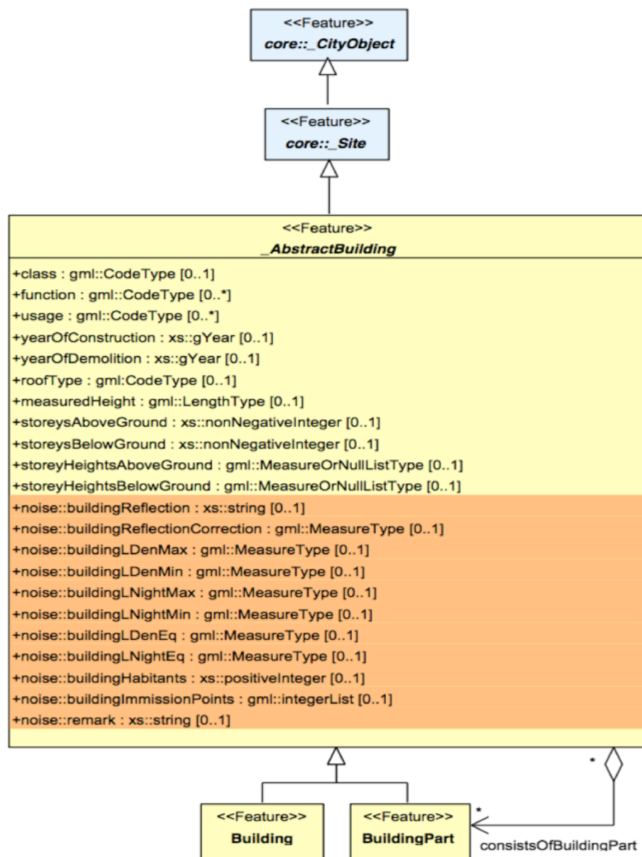
Fig. 1 Excerpt of the UML diagram of the Noise ADE, depicting the augmentation of CityGML Building with noise related attributes not standardly available in CityGML. The prefix noise indicates attributes and objects that are associated with the Noise ADE. Source: OGC CityGML 2.0 standard [1]
