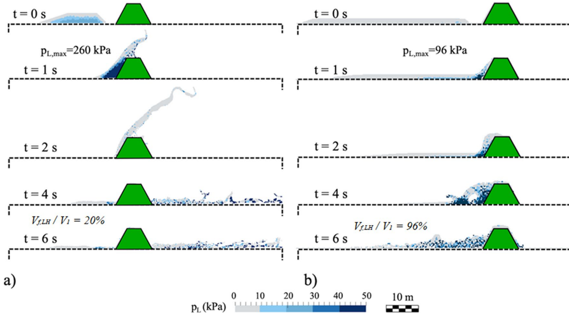
Fig. 13 Pore-water pressure distribution for different flows: a v_0 = 20 m/s (case 2); b H/h = 6 (case 4)
