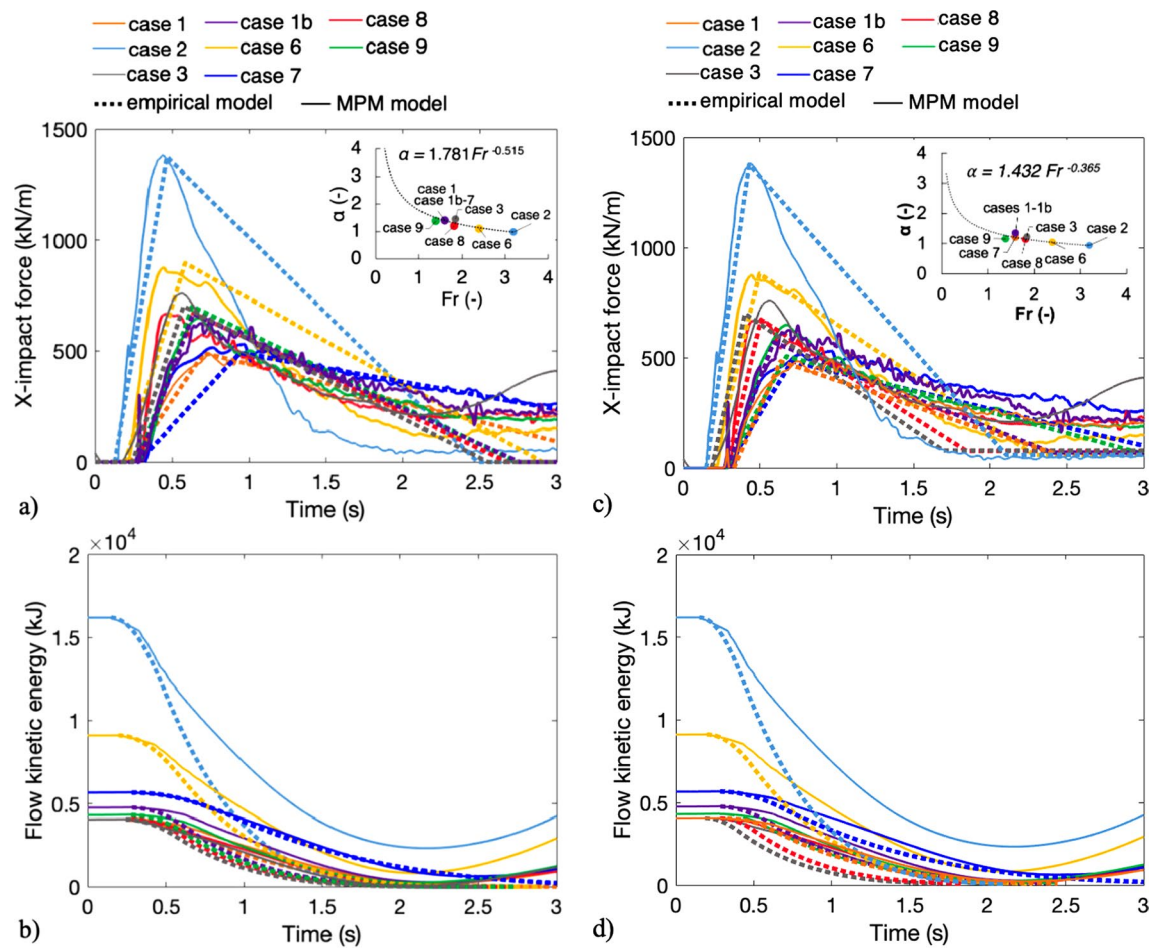
Fig. 8 Calibration of the empirical model through the MPM simulations (for the cases in Table 2): impact force (a) and kinetic energy (b) time trend for \kappa = 0 and impact force (c) and kinetic energy (d) time trend for \kappa = 1
