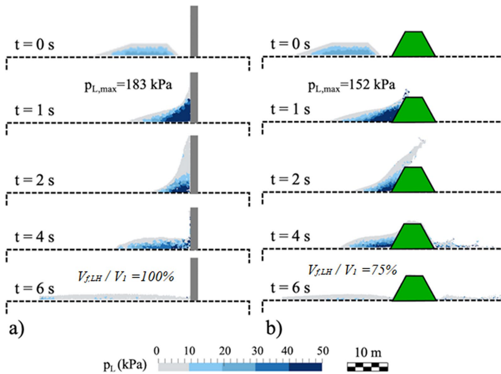
Fig. 12 Pore-water pressure distribution for: a infinite wall (case 3); b fixed barrier (case 1)
