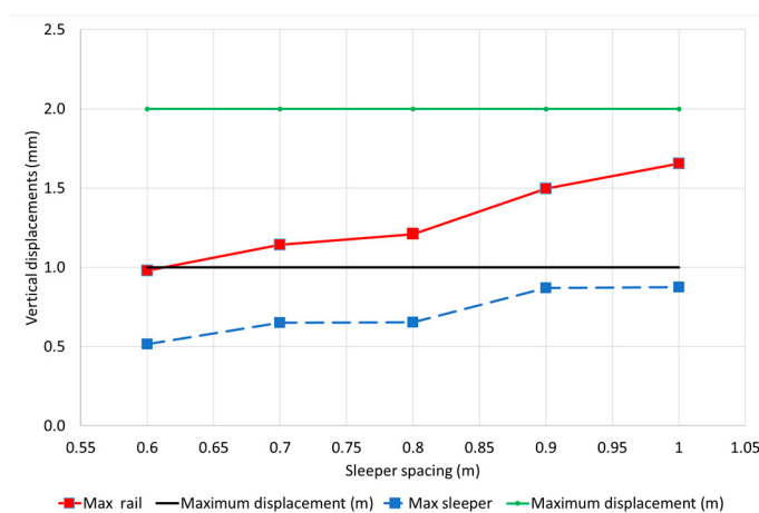
Figure 10. Maximum allowed limits for vertical displacements on rails and sleepers according to Table 7 values.
