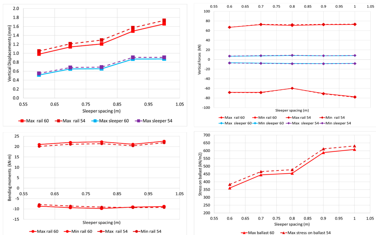
Figure 5. Case 3. Maximum vertical displacements of the rail and sleeper, vertical forces on rail and sleeper, rail bending moments, and stresses on ballast.
