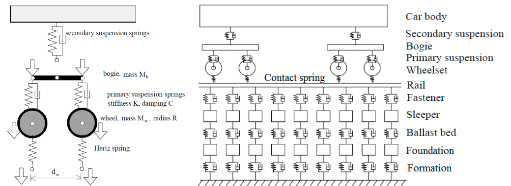
Figure 2. Simplified model. Train model (left). Couple model of train and track as a combination of springs and dampers (right).
