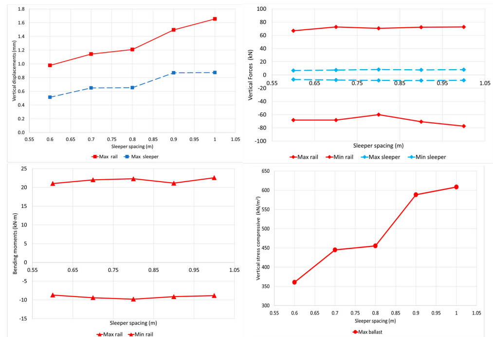
Figure 3. Case 1. From left to right, and from top to bottom. Maximum vertical displacements of the rail and sleeper, vertical forces on rail and sleeper, rail bending moments, and stresses on ballast.
