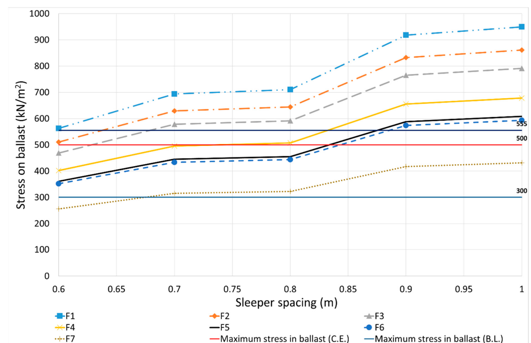
Figure 12. Importance of effective area considered under sleeper. It is important in order to calculate the stress in the ballast surface just under the sleeper.
