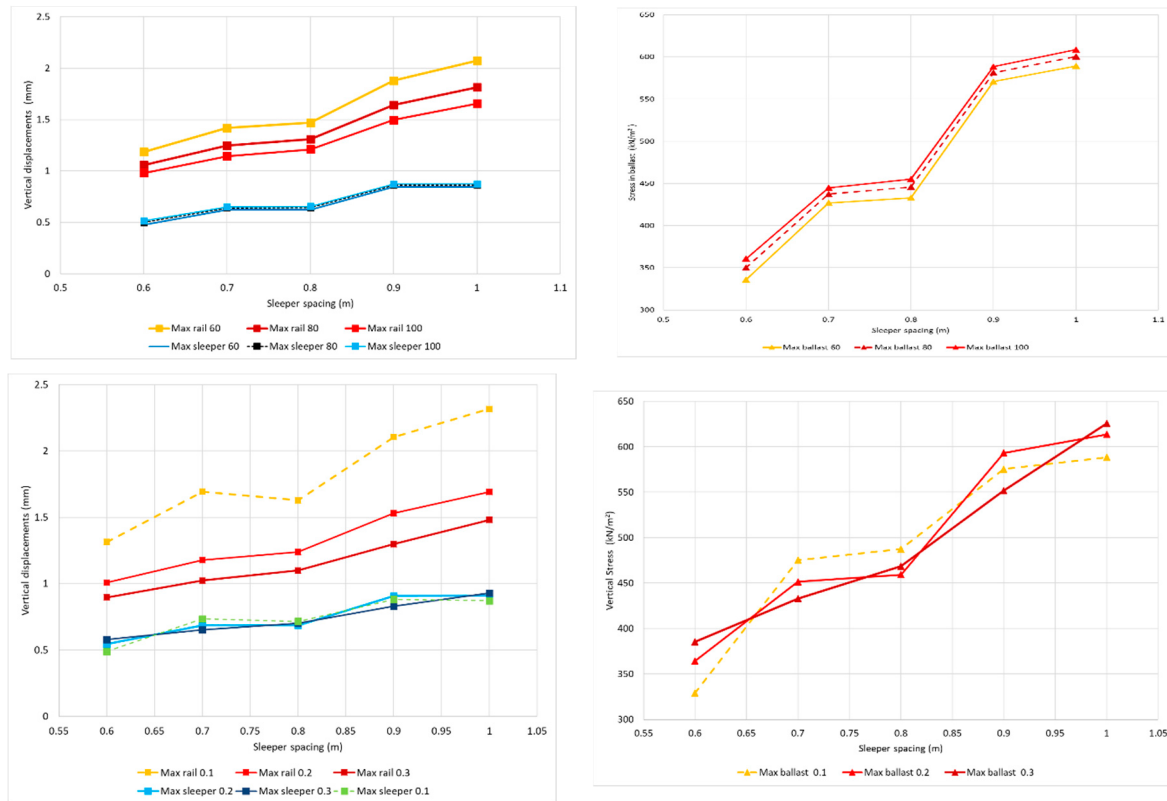
Figure 9. Case study with different pad materials (up) and different geometry (down).
