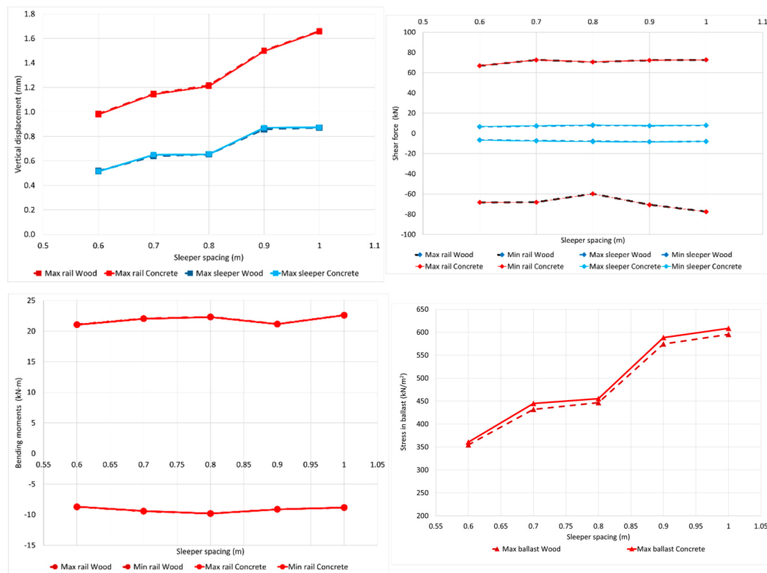
Figure 6. Case 4. Maximum vertical displacements of the rail and sleeper, shear forces on rail and sleeper, rail bending moments, and stresses on ballast.
