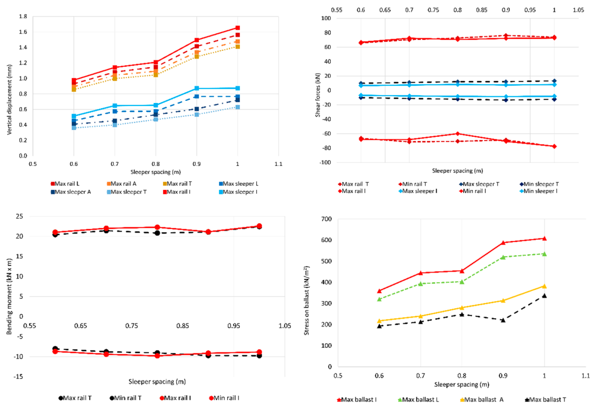
Figure 7. Case 5. Maximum vertical displacements of the rail and sleeper, shear forces on rail and sleeper, rail bending moments, and stresses on ballast (A—change the sleeper width, L—change the sleeper length, T—change both width and length, I—initial size of the sleeper).
