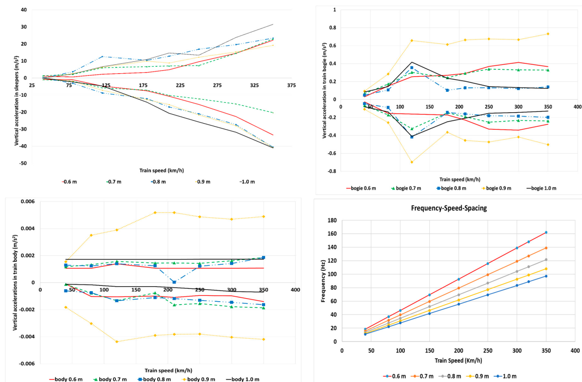
Figure 4. Case 2. Maximum and minimum vertical accelerations in the sleepers ( up, left ), in the bogie ( up, right ), and in the train ( down ) for the speeds studied and the defined spacings. Frequency with train speed and sleeper spacing variation ( down, right ).
