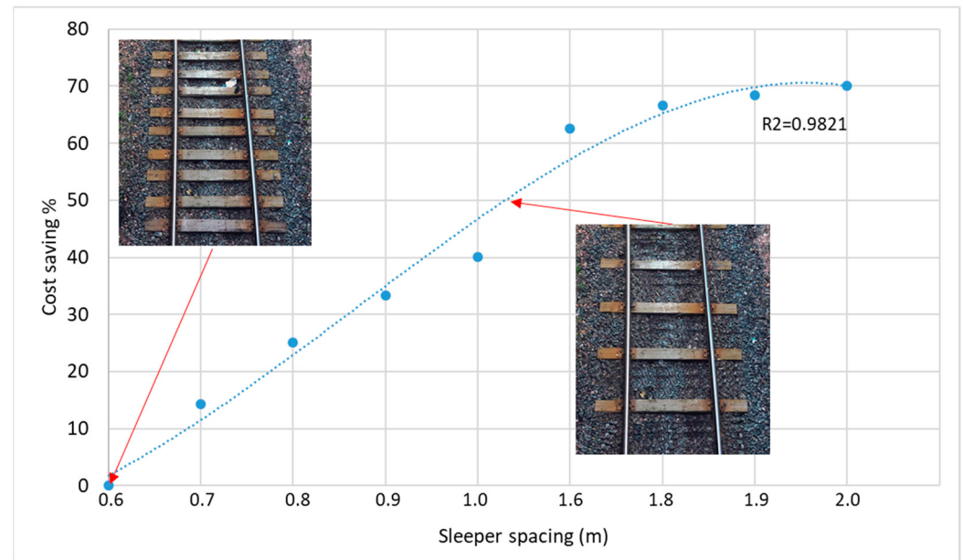
Figure 1. Cost savings estimation in terms of sleepers spacing.
