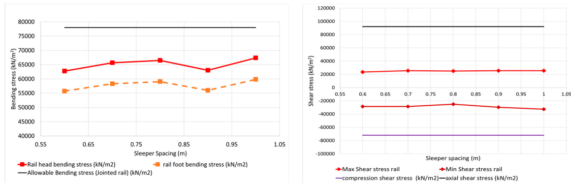
Figure 11. Maximum allowed shear stress and bending stress in rails according to Table 7 values.
