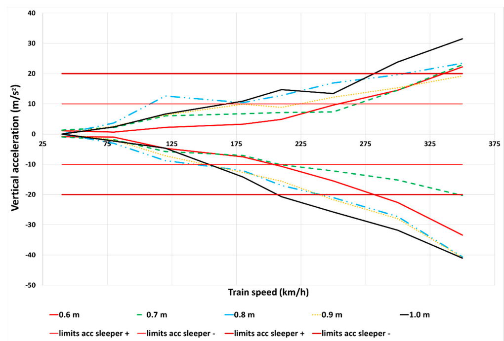
Figure 13. Limits for vertical acceleration on sleepers.
