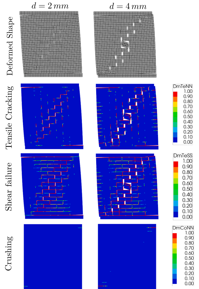
Fig. 8. The deformed profile, and damage plots indicating tensile, shear and crushing failures for the pushover study of reference discrete-crushing model, with discrete cracking-shearing-crushing interfaces, using SLA at 2 mm and 4 mm prescribed lateral displacements.
