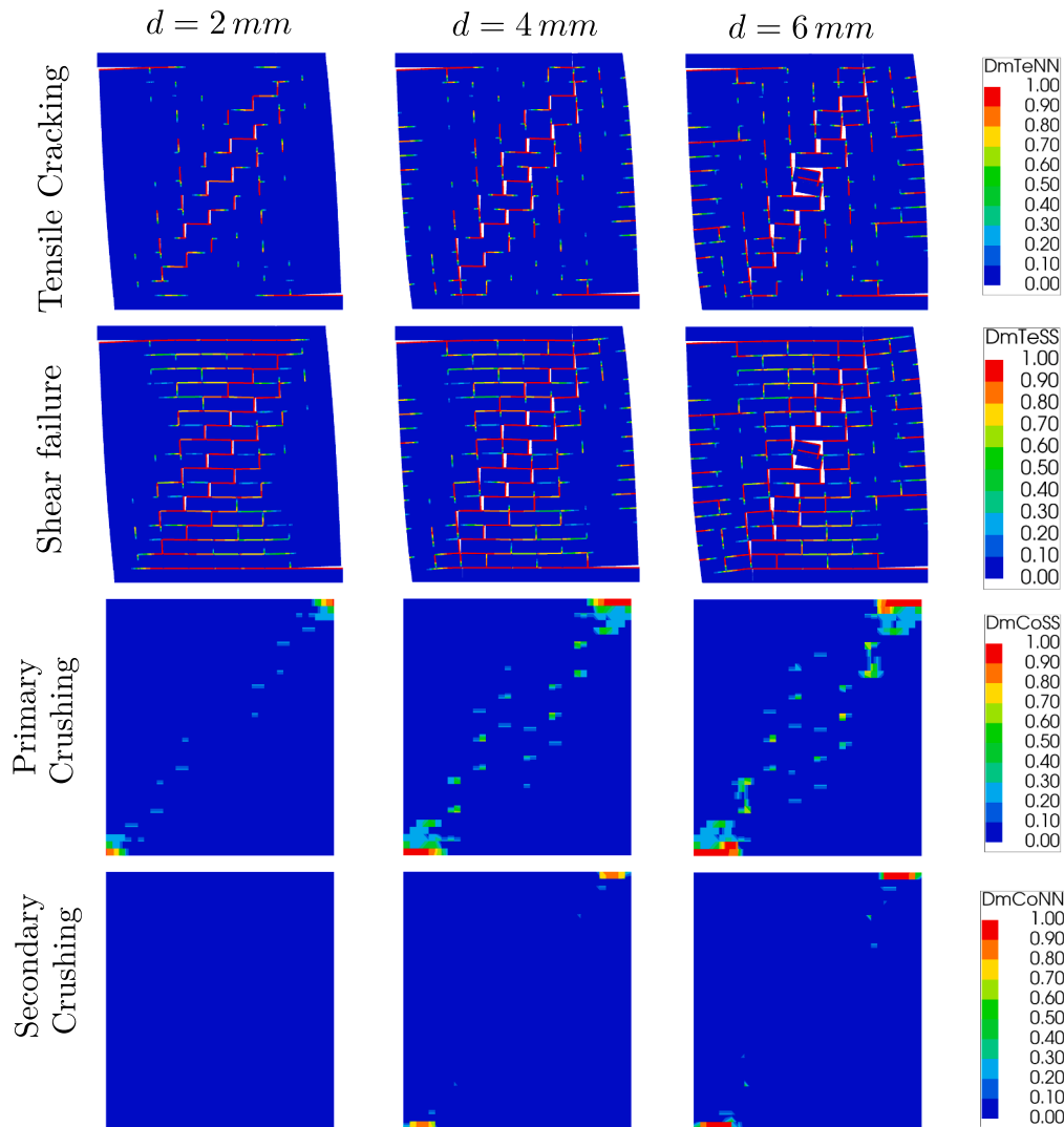
Fig. 15. Damage plots indicating tensile, shear and crushing failures for the pushover study of the smeared-crushing model, with discrete cracking and shearing in interfaces while crushing is smeared in the continuum, using SLA at 2 mm, 4 mm and 6 mm prescribed lateral displacements.
