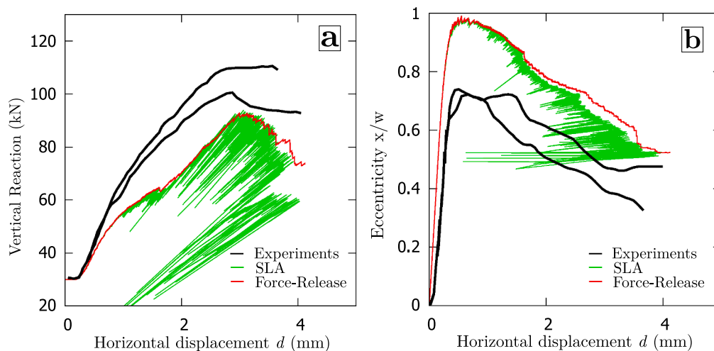
Fig. 9. (a) Evolution of the vertical reaction forces and (b) its eccentricity with respect to the center line of the wall, for increasing prescribed lateral displacements in the SLA and Force-Release simulations (discussed under Case-2 of the section on variation studies) of the discrete-crushing model.
