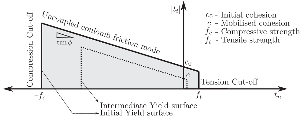
Fig. 2. Failure surface for the 2D line interfaces.
