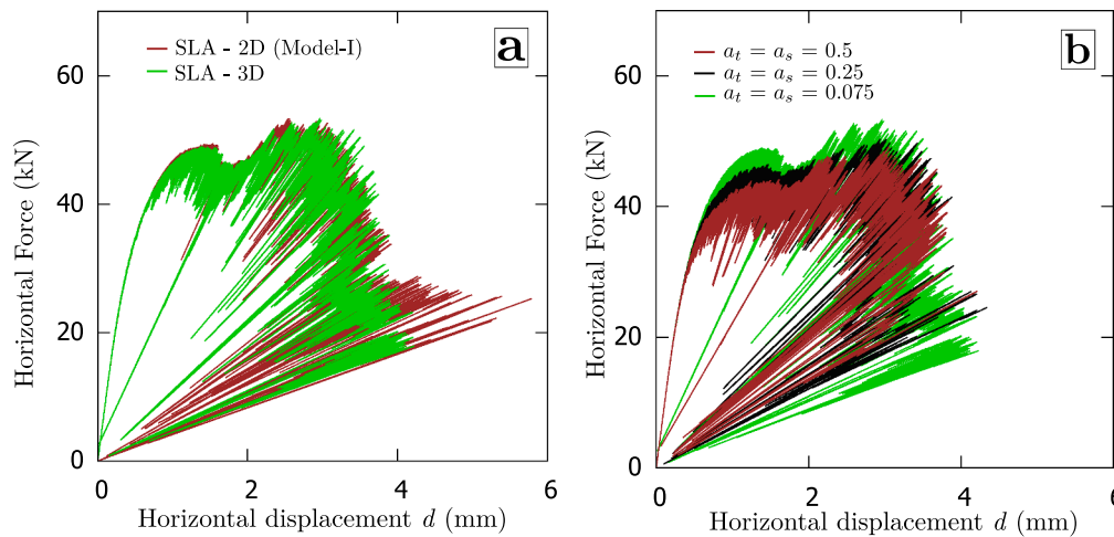
Fig. 18. Force–displacement curves of the 2D and 3D SLA simulations, (b) 3D SLA simulations for varying values of user-specified shear displacement increment factors a_t and a_s .
