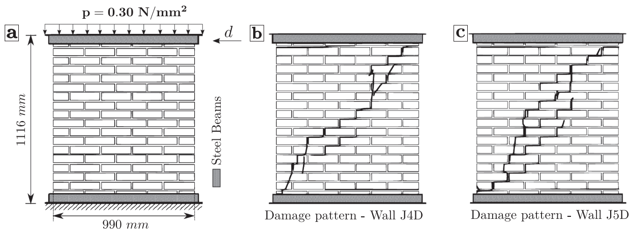
Fig. 5. (a) Schematic representation of solid clay brick masonry walls (J4D & J5D), loaded firstly by an overburden pressure of 0.30 N/mm 2 followed by a lateral prescribed displacement d ; and the experimental crack patterns of the walls (b) J4D and (c) J5D.
