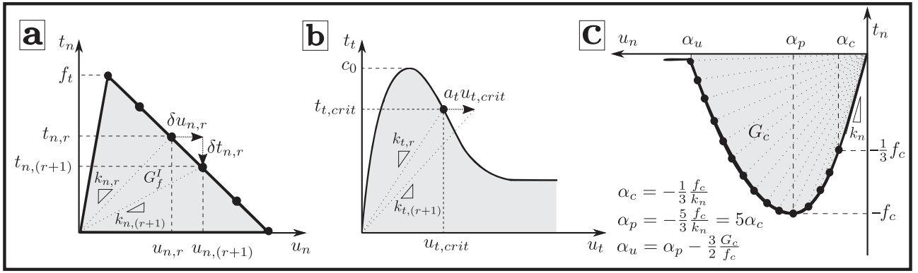
Fig. 3. (a) Linear tension softening law evolving 'during' analysis with user specified relative normal displacement increments, (b) cohesion softening law deduced 'during' analysis with user specified relative shear displacement increments, and (c) pre-defined parabolic hardening-softening saw-tooth law for compression [29]. Studies in this article use (b) as such for the shear mode, while predefined band width ripple versions of (a)&(c) (Fig. 1) are used for tension and compression.
