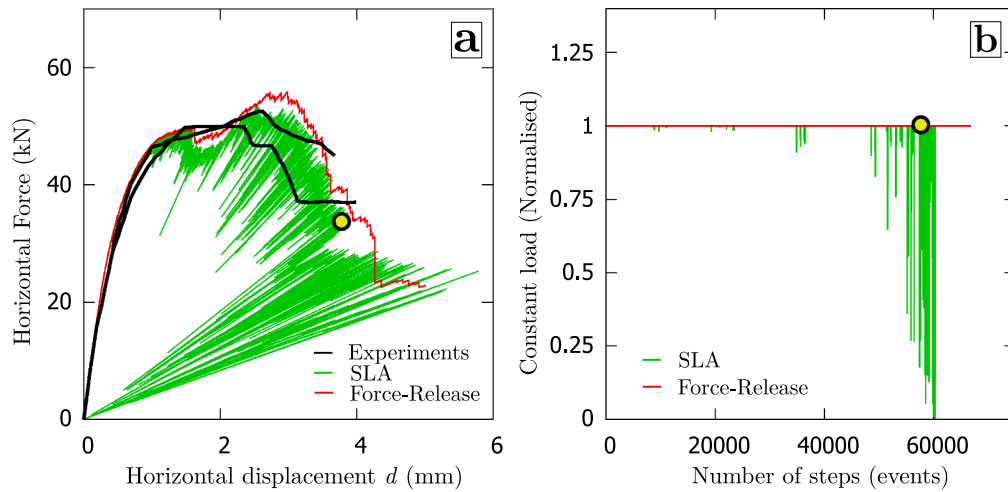
Fig. 12. Force–displacement curves of the experiments compared against those of the SLA and the Force-Release simulations of the discrete-crushing model, and (b) the evolution of constant load of precompression during the simulations.
