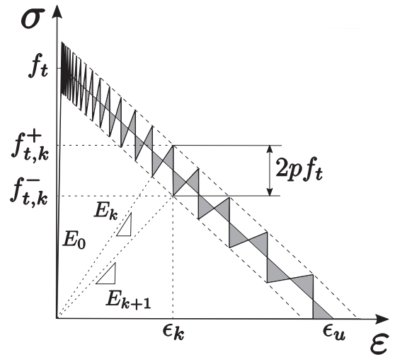
Fig. 1. Linear tension softening saw tooth law, with p the saw-teeth discretisation factor, based on the band width ripple approach to ensure mesh objectivity [15]. In this approach, a strength range p is defined as a percentage of the undamaged material strength f_t and a band is introduced into the softening part of the base curve, enclosing it such that the upper and lower triangles cancel each other out to eventually yield the same fracture energy.
