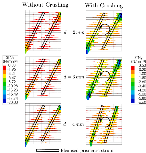
Fig. 11. Evolution of compressive tractions along bed joints of the wall, with and without the crushing failure possibility (note the different colour scales), for increasing lateral displacements and the schematic view of the rotation and movement of two parallel struts in the case of crushing failure possibility, with progressive crushing of the toe region of the wall.
