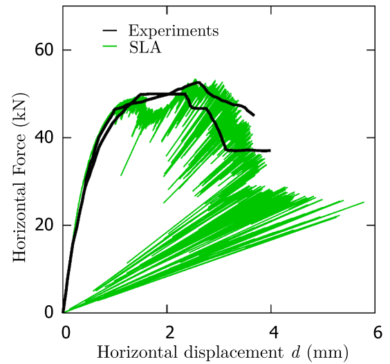
Fig. 7. Force-displacement curves of the experiments compared against those of SLA for the reference micro model with discrete cracking, shearing and crushing in interfaces.
