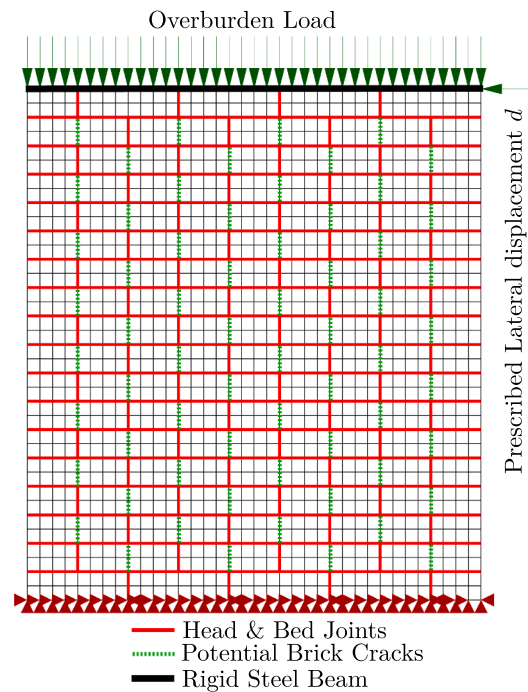
Fig. 6. 2D Finite element micro model of the solid clay brick wall subject to overburden and pushover loads.
