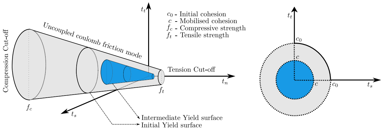
Fig. 4. Failure surface for the 3D planar interfaces.
