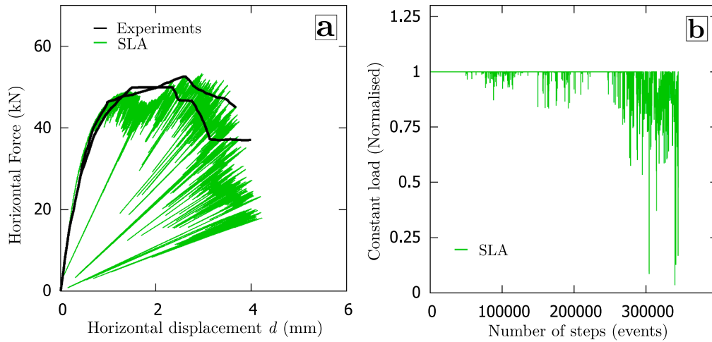
Fig. 17. Force–displacement curves of the experiments compared against those of the SLA for the 3D model, and (b) the evolution of constant load of precompression during the SLA simulation.
