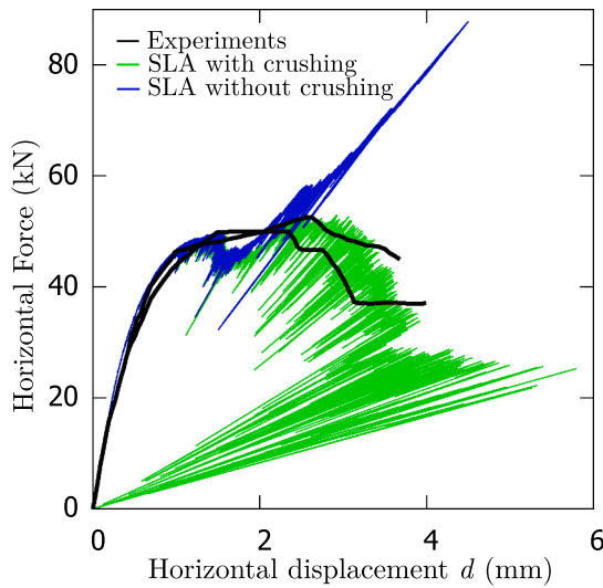
Fig. 10. Force-displacement curves of the SLA simulation of the micro models with and without crushing nonlinearities.
