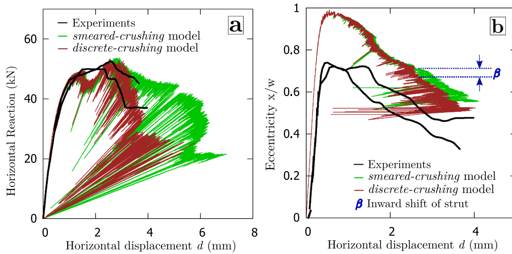
Fig. 14. (a) SLA simulations of the discrete-crushing model, and the smeared-crushing model with compression nonlinearity smeared into the continuum, and (b) evolution of eccentricity of vertical reaction forces up to 4 mm horizontal displacement.
