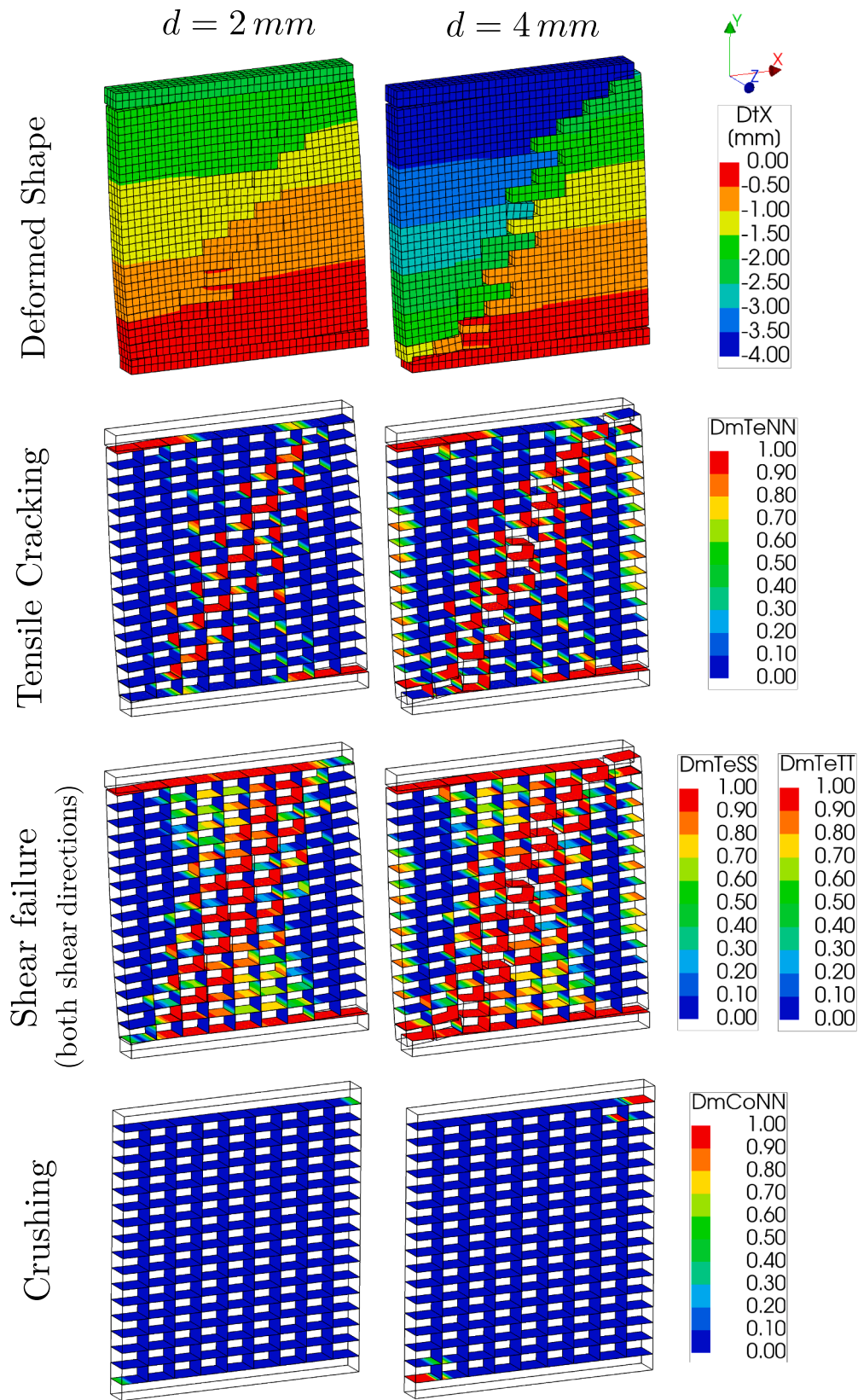
Fig. 19. Deformed profiles, and damage plots indicating tensile, shear and crushing failures for the pushover study of 3D Model using SLA at 2 mm and 4 mm prescribed lateral displacements.
