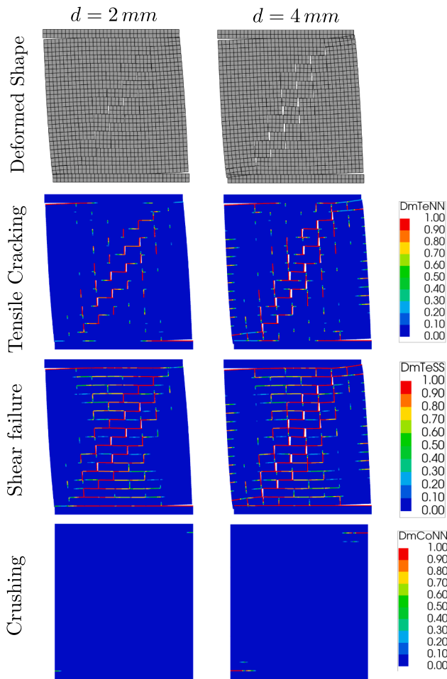
Fig. 13. The deformed profile, and damage plots indicating tensile, shear and crushing failures for the pushover study of reference discrete-crushing model, with discrete cracking-shearing-crushing interfaces, using the Force-Release method at 2 mm and 4 mm prescribed lateral displacements.
