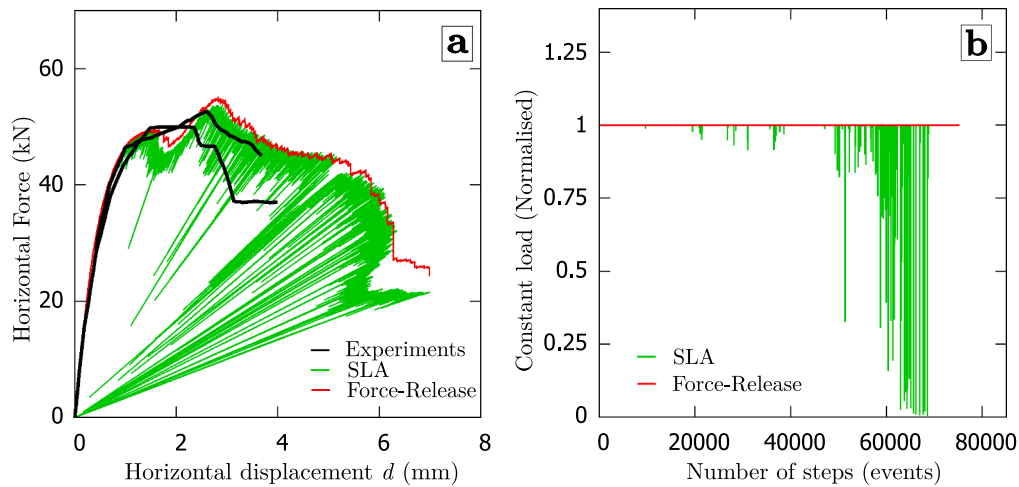
Fig. 16. Force–displacement curves of SLA and the Force-Release simulations of the smear -crushing model, and (b) the evolution of constant load of precompression during the simulations.
