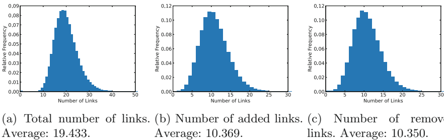
Fig. 4. Histograms of link statistics for the reduced MMP model with 25 nodes across 1000 realizations of 1000 time steps.
