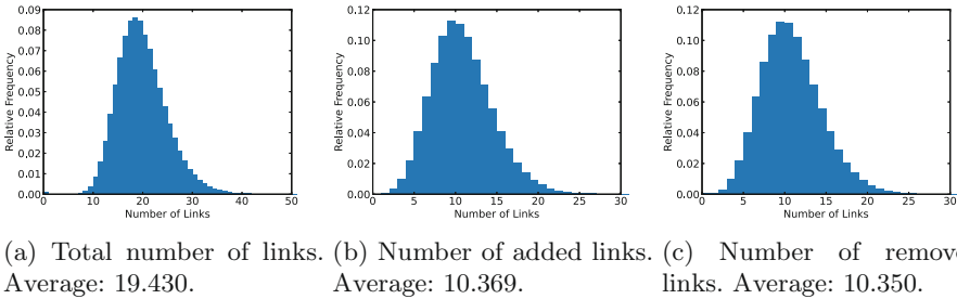
Fig. 3. Histograms of link statistics for the simulated mobility process with 25 nodes across 1000 realizations of 1000 time steps.
