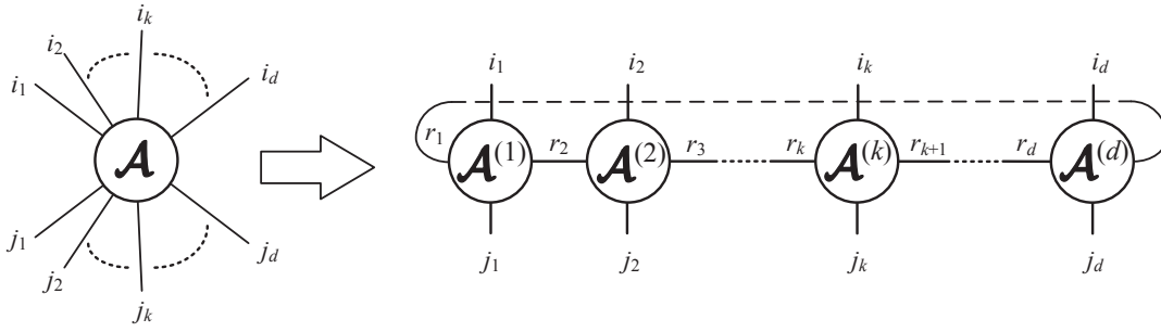
Fig. 3: Matrix product operator (MPO) decomposition.
