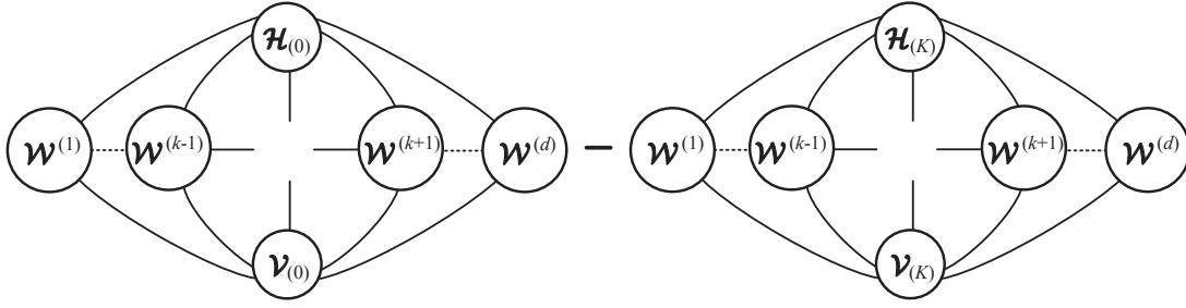
Fig. 5: The derivative of the log-likelihood function with respect to the k th MPO-core \mathcal{W}^{(k)} .
