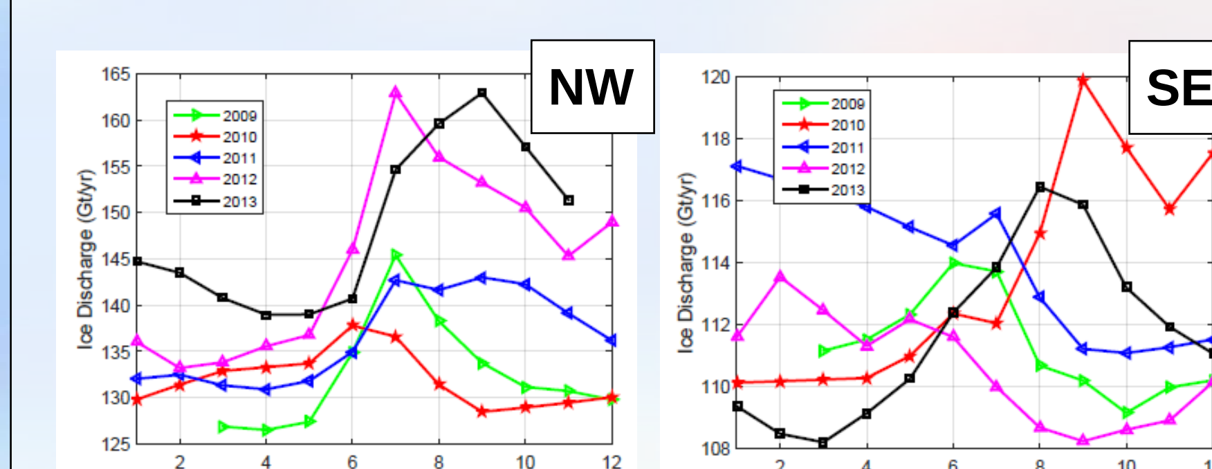
Fig.5 Temporal variations in ice discharge in 2009–2013 obtained by the summation of estimates for individual marine-terminating glaciers located in the NW (left) and SE (right) drainage system. Locations of the considered glaciers are depicted with red dots in Fig.1 (55 glaciers in total). The observed variations stay within 10–20%.
