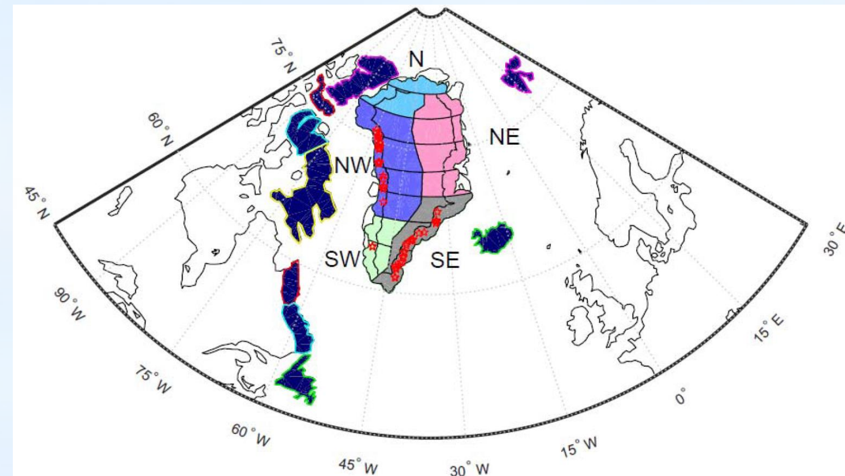
Fig.1 The territory of Greenland is panelized into 28 mascons, which are aggregated into five drainage systems. In addition, 9 mascons outside Greenland are defined to account for possible mass variations there. Red stars denote the glaciers considered in the estimation of ice discharge (see Sect. 8)
