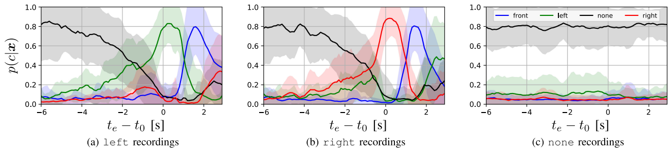
Fig. 8. Mean and std. dev. of predicted class probabilities at different times t_e on test set recordings of the Static data (blue is front , green is left , red is right , and black is none ). Each figure shows recordings of a different situation. The approaching vehicle appears in view just after t_e - t_0 = 0 .
