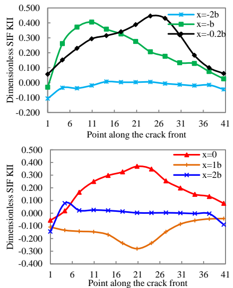
Fig. 7. The histories of K_{II} along the crack tip at three wheel locations (a) before reaching the crack mouth, (b) after passing the crack
