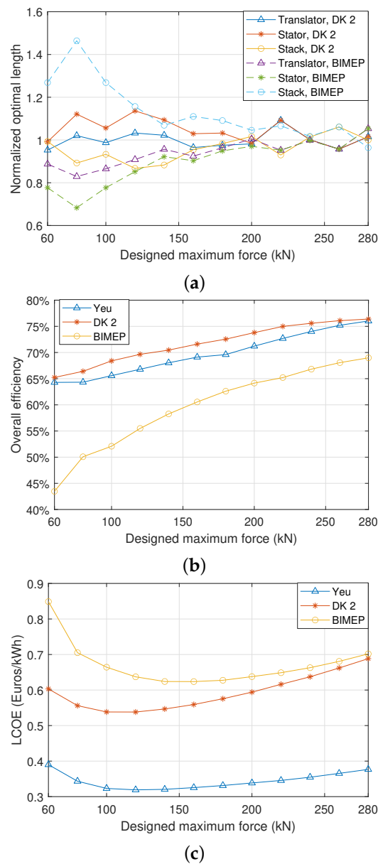
Figure 11. The optimized design parameters, the overall efficiency and the LCOE of the WEC with various designed maximum forces in three different wave sites. (a) The optimized design parameters for DK 2 and BIMEP, which are normalized to the corresponding values in Yeu island. (b) The overall efficiency of the linear generator as a function of the designed maximum generator force. (c) The LCOE of the WEC as a function of the designed maximum generator force.
