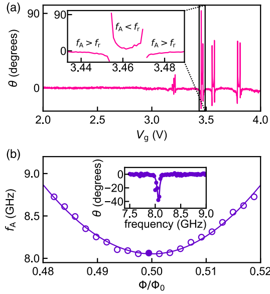
FIG. 3. Control of the Andreev qubit frequency. (a) The average phase \theta of the readout tone for a range of V_g values ( \Phi = \Phi_0/2 ). Each point was integrated for 1.28 \mu s. As V_g is varied, transitions in the nanowire come into proximity with the resonator frequency, resulting in avoided crossings. Inset: enlargement of two of these avoided crossings of f_A with the resonator frequency. (b) Inset: Continuous-wave two-tone spectroscopy reveals the qubit transition. The transition frequency f_A is extracted from a best fit to a Lorentzian line shape. Main figure: dependence of f_A on \Phi . Solid line is a fit to the short-junction formula for f_A [31].
